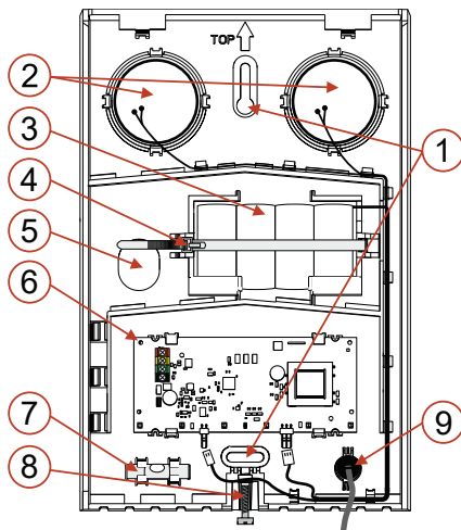
Figure 1: Description of internal parts of the product
