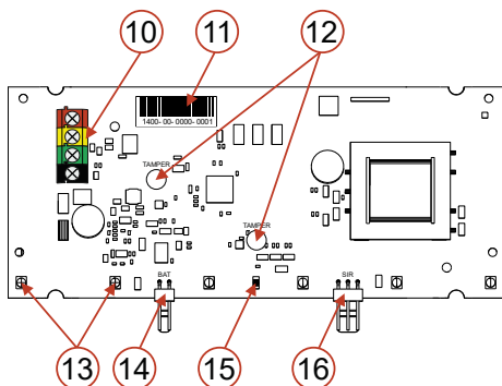
Figure 2: Description of printed circuit board
