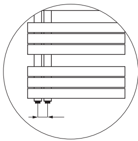
Detail of the pipe centres 50 mm version
