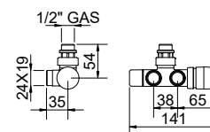
VALVE KRISTAL BIDIRECTIONAL SQUARE LEFT WHITE R01
