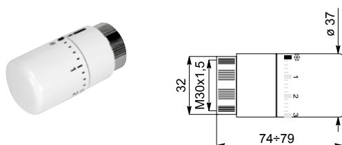
WHITE THERMOSTATIC HEAD
