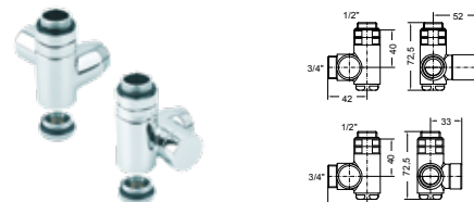
KRISTAL VALVE COMBI WITH THERMOSTATIC OPTION - CHROMED FINISHING
