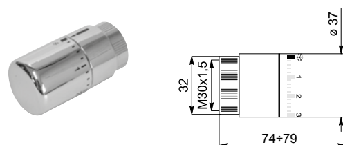
CHROMED THERMOSTATIC HEAD
