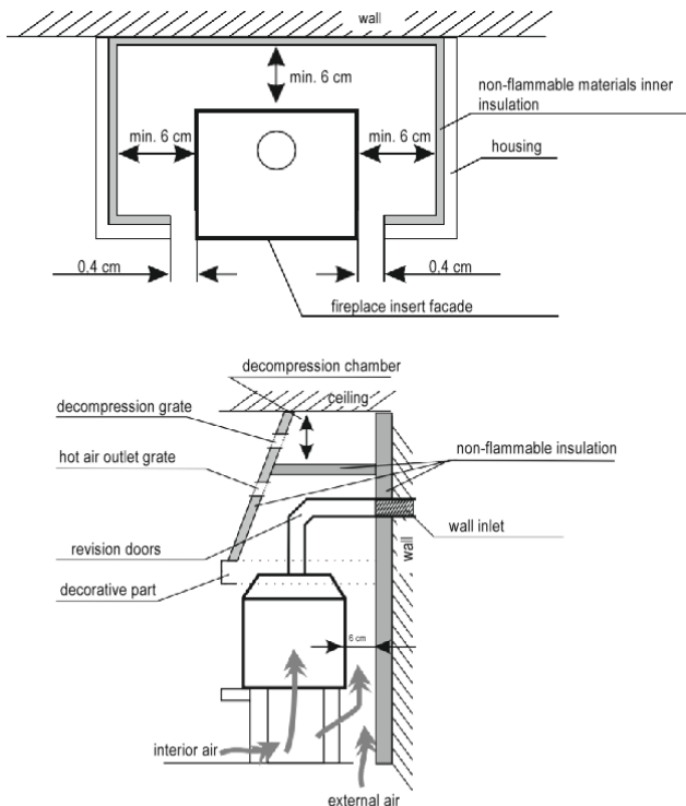
Fig. 3. Example of installing the fireplace insert - top and side.
