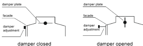
Fig. 5. The example of the damper adjustment
