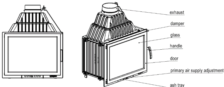
Fig.1. Fireplace insert schematics
