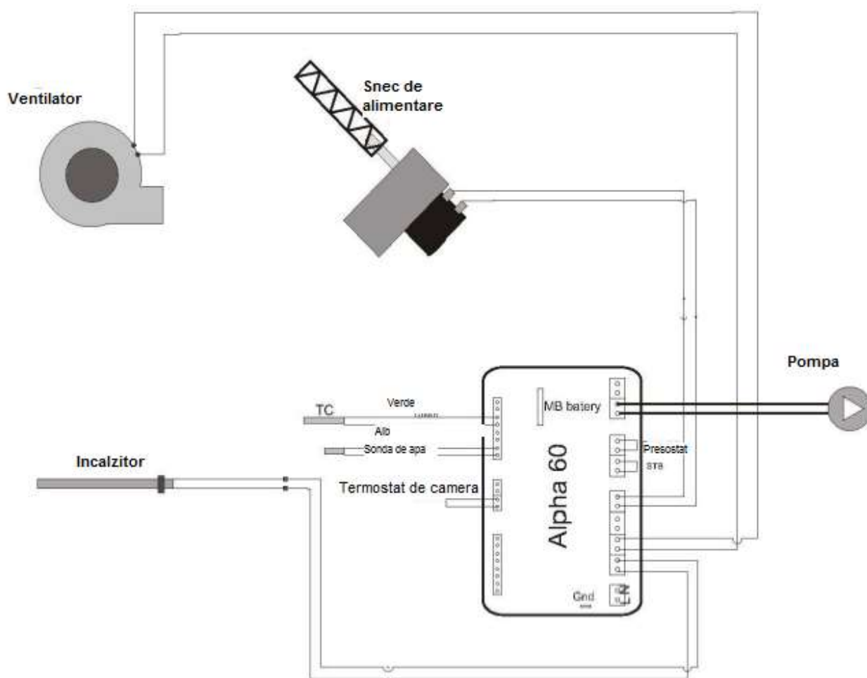
Figura 30: Schema electrica
