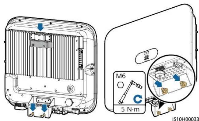
Figura 4-11 Instalarea SUN2000
