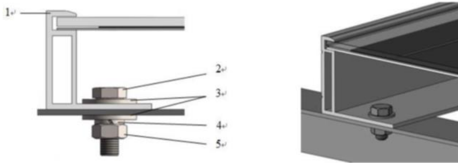
Fig.1 Backsheet-Glass module
