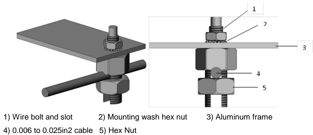
Figure 4. Tyco grounding bolt # 2058729-1
