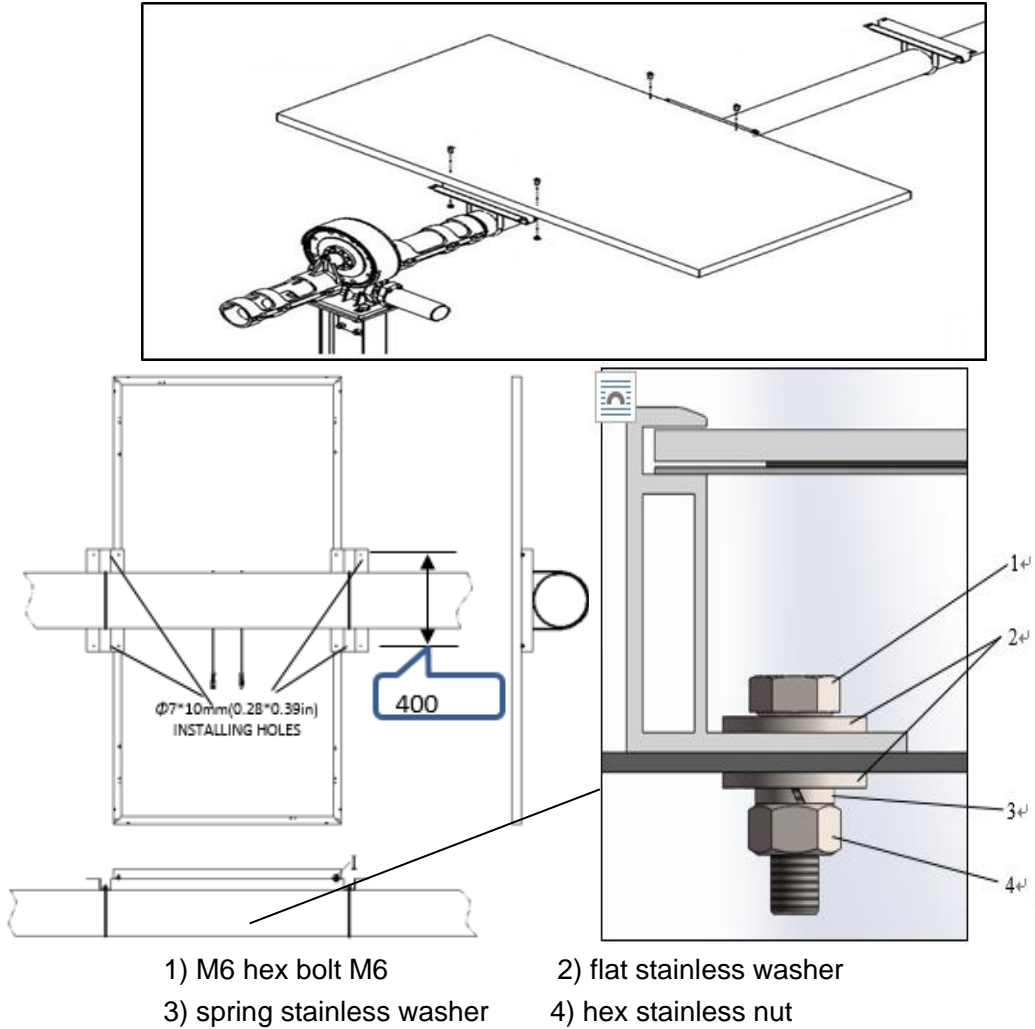
Fig 2. Backsheet-Glass module with Single-axis Tracing System
