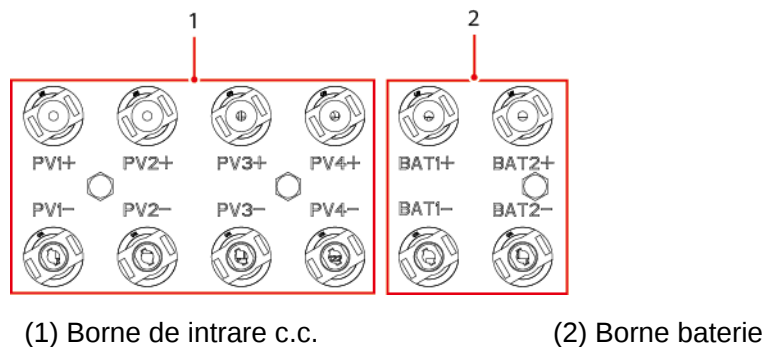
Figura 5-11 Borne
