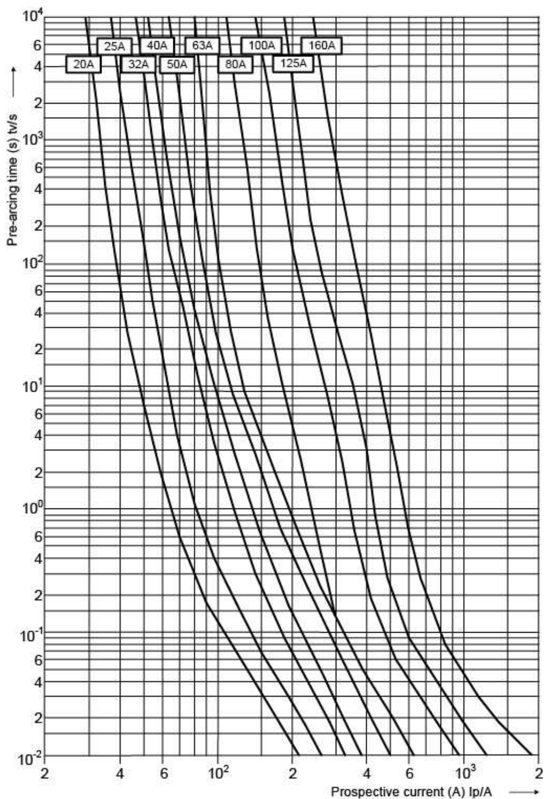
Time-current characteristics NH00C and NH00
