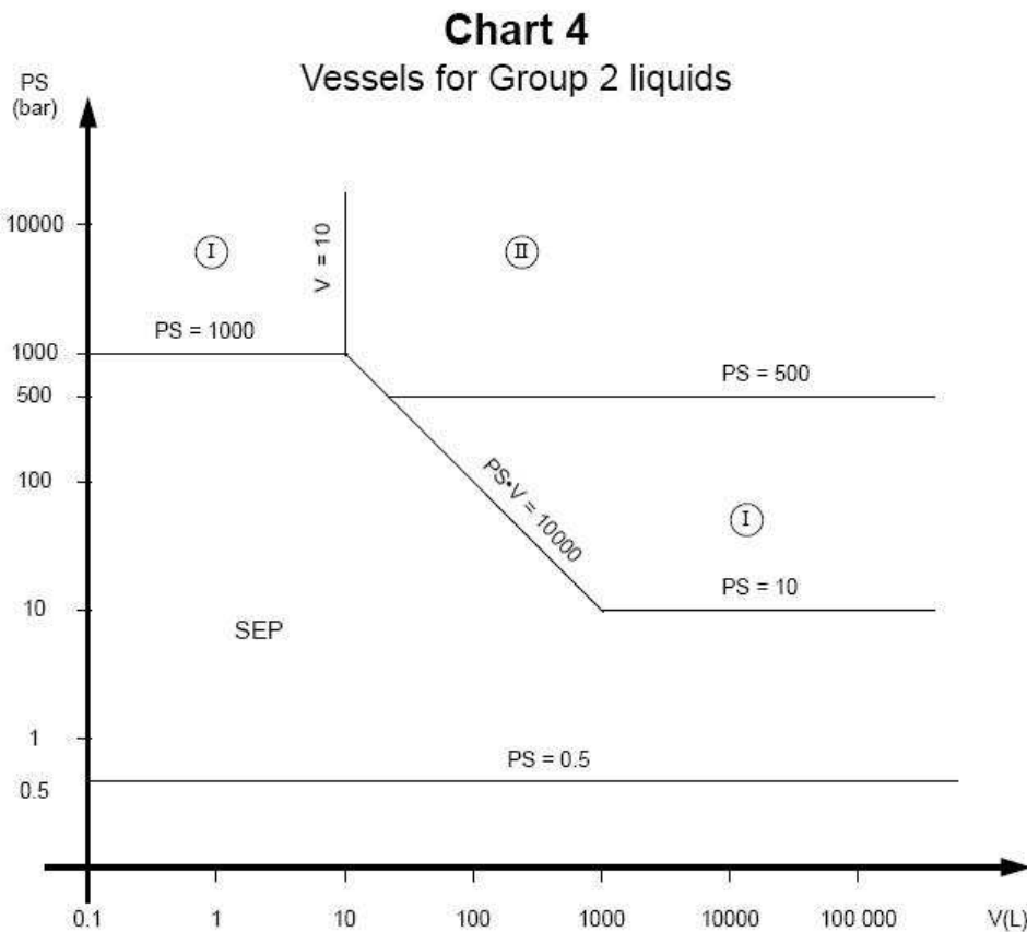
Figure 1: Pressure Equipment Category (Ref. PED 97/23/EC)
