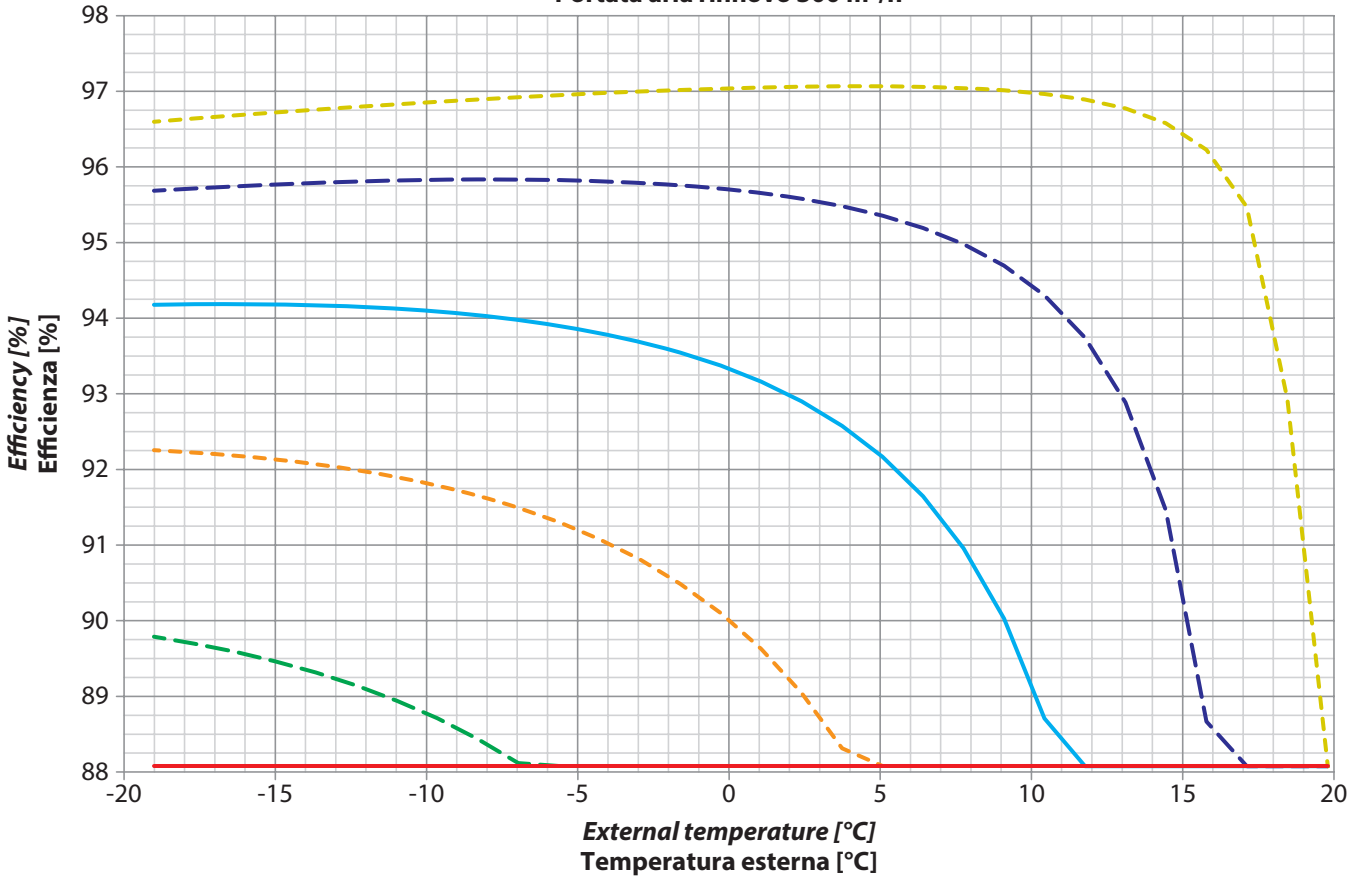
Renewal air flow rate 300 m 3 /h Portata aria rinnovo 300 m 3 /h
