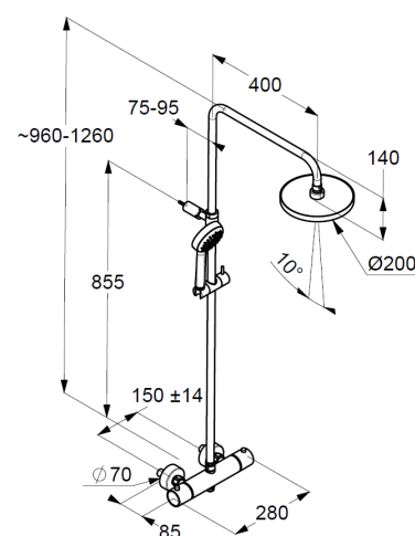
Dimensional drawing
