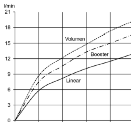
Flow rate diagram
