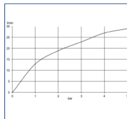
Diagrama debit
