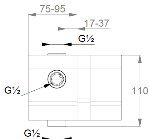
Dimensional drawing
