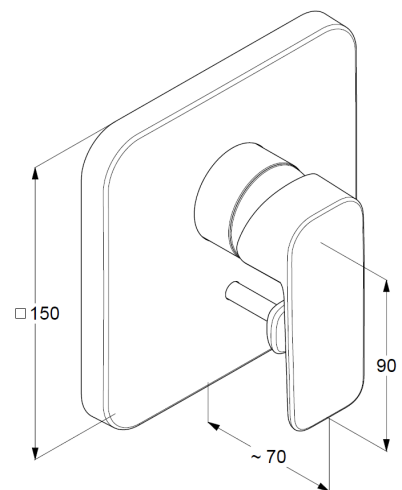
Dimensional drawing
