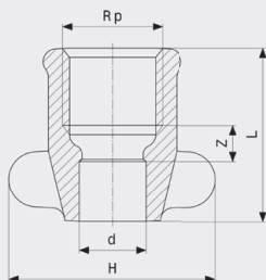
Adapter - gunmetal Model 94270GF
