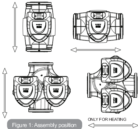
Figure 1: Assembly position
