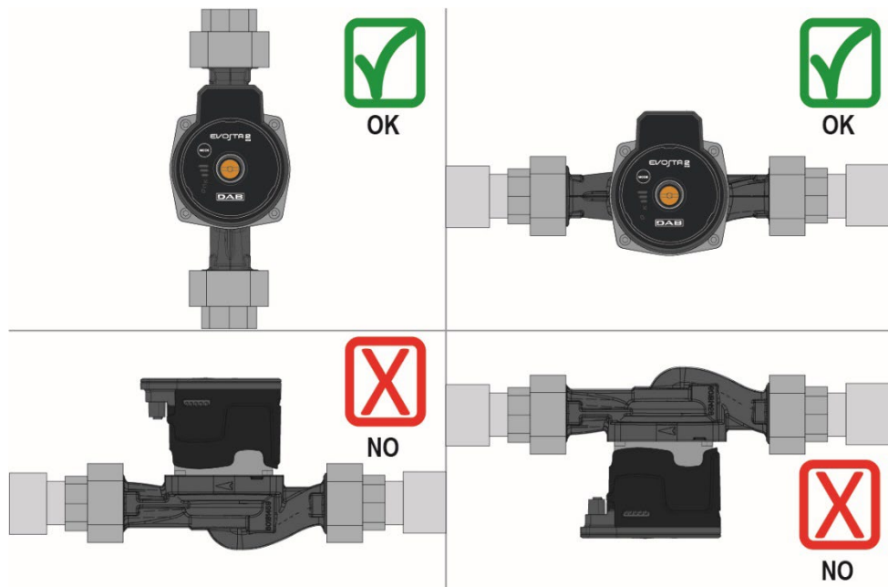
Figure 3: Assembly position
