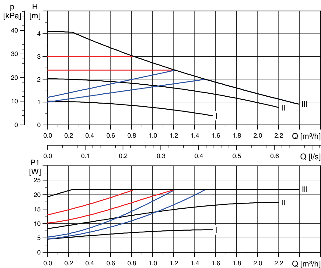
Fig. 18 Curbe caracteristice, ALPHA2 L XX-40
