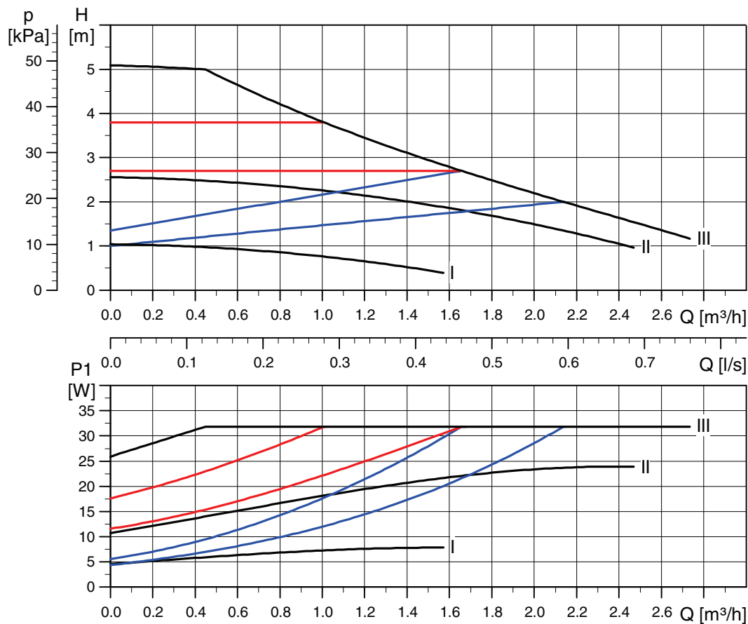
Fig. 20 Curbe caracteristic, ALPHA2 L XX-50
