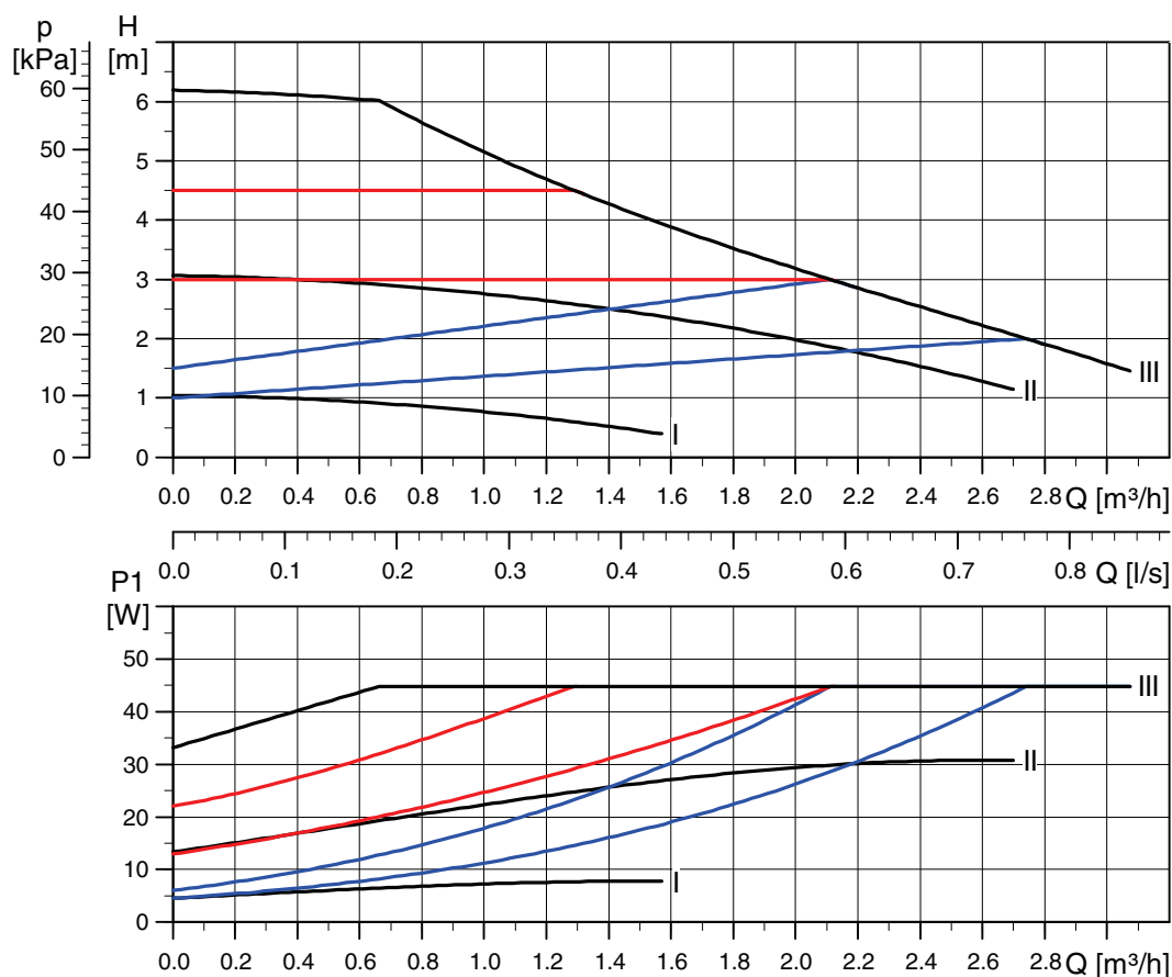
Fig. 21 Curbe caracteristic, ALPHA2 L XX-60
