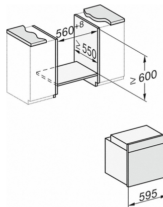
H226x-1B/BP/E/EP/I/IP, H2x6xB/BP, H7x6xB/BP/BPX, schițe de instalare
