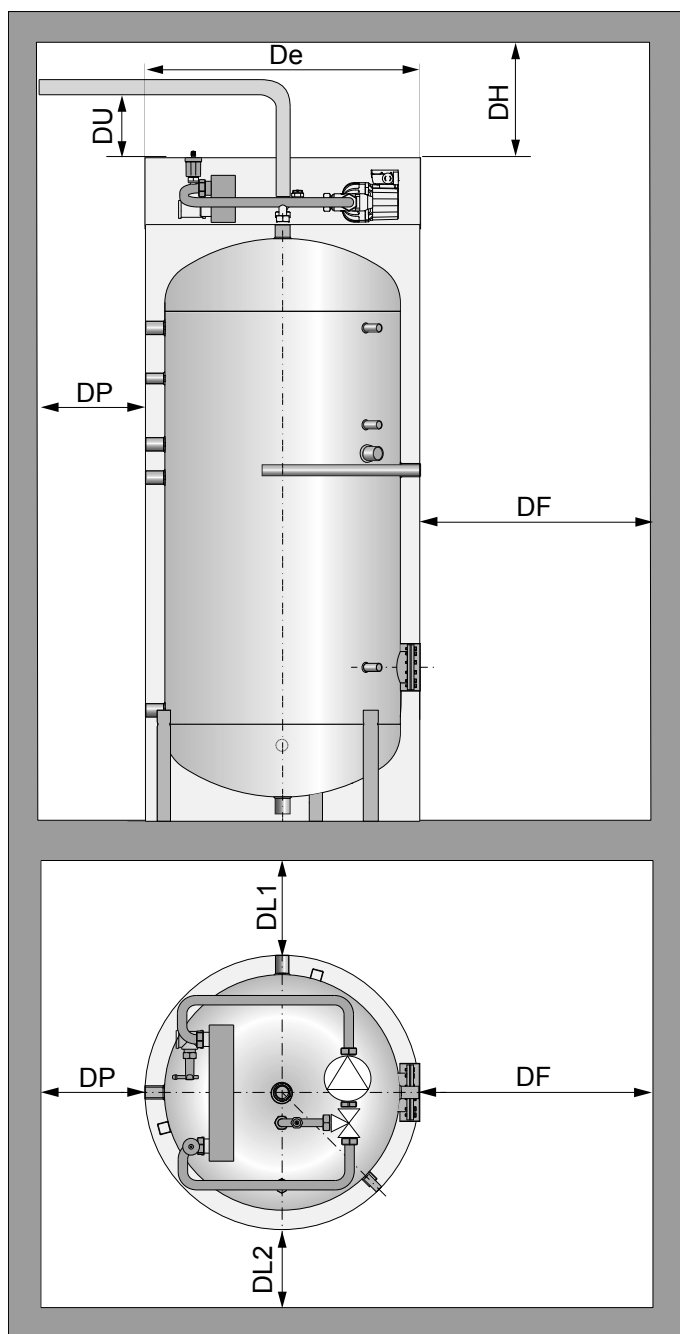
Illustration 1 - Distances minimum:
