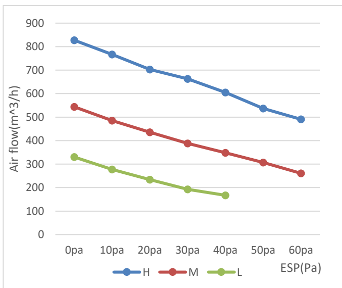
MKT4-400FG30-CL
