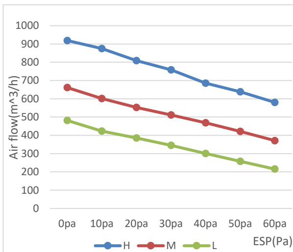
MKT4-400FG50-CL
