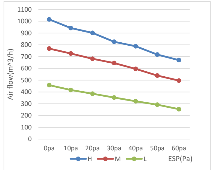
MKT4-500FG30-CL
