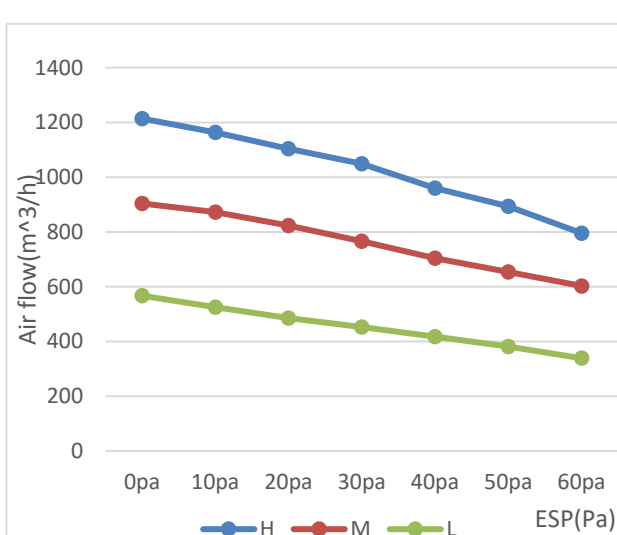
MKT4-600FG50-CL
