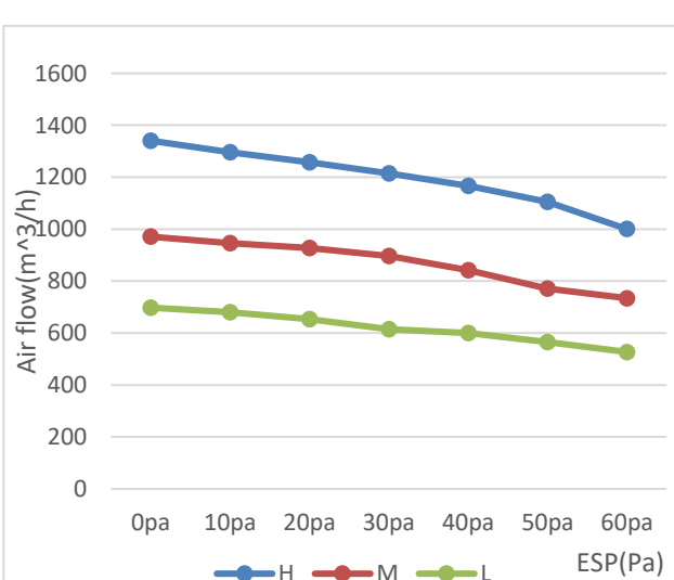
MKT4-700FG50-CL
