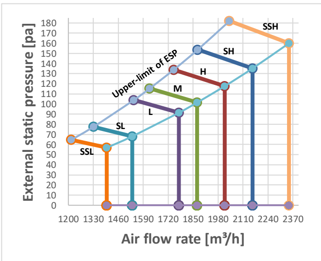
Figure 9.13: MIH160T2N18
