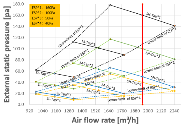
Figure 9.23: MIH112T2N18
