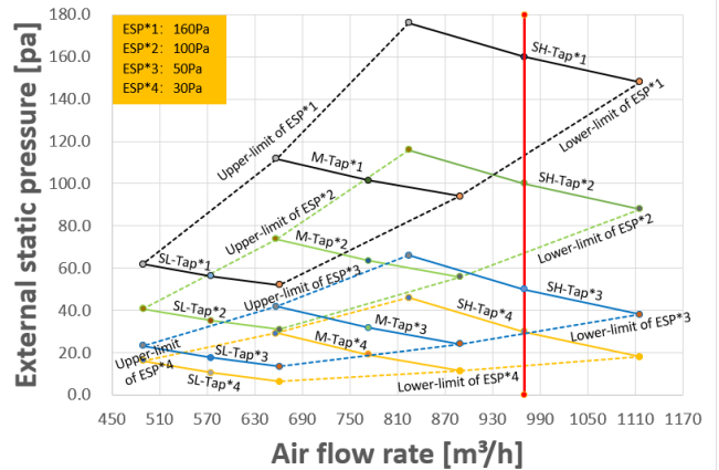
Figure 9.19: MIH56T2N18
