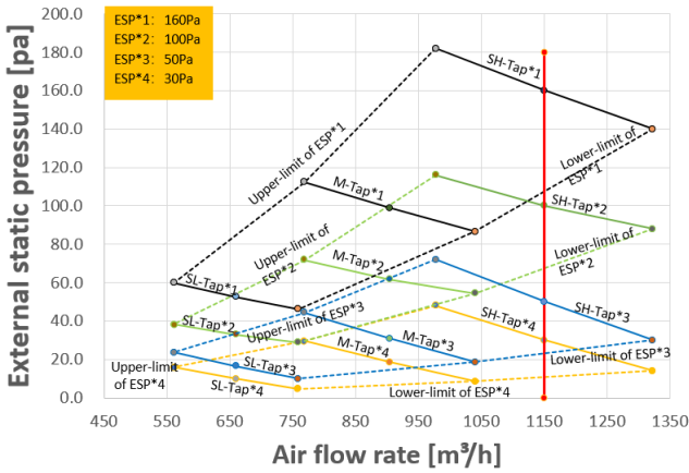
Figure 9.20: MIH71T2N18
