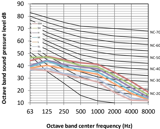
Figure 8.15: MIH160T2N18 octave band levels
