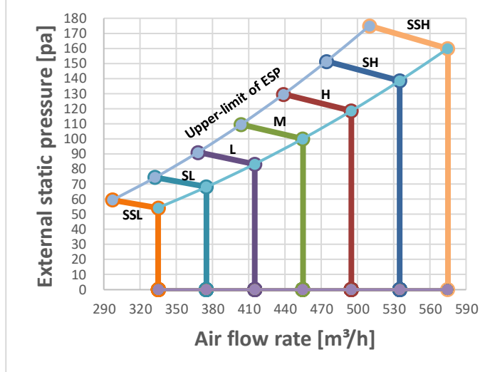
Figure 9.4: MIH36T2N18
