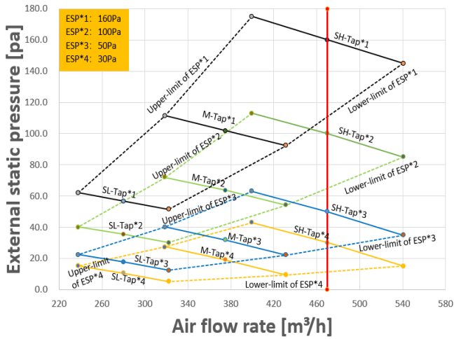
Figure 9.14: MIH15T2N18
