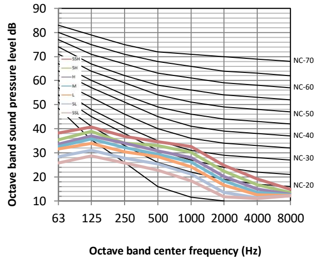
Figure 8.10: MIH80T2N18 octave band levels
