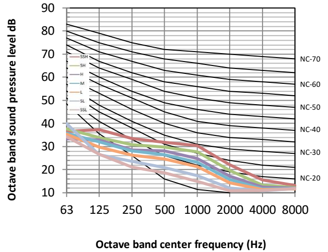
Figure 8.8: MIH56T2N18 octave band levels
