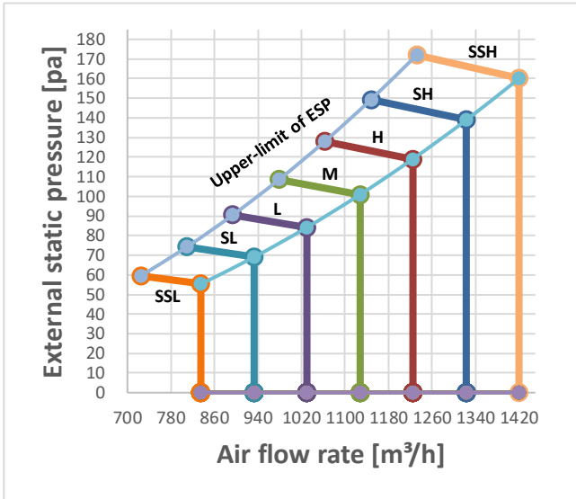
Figure 9.9: MIH90T2N18
