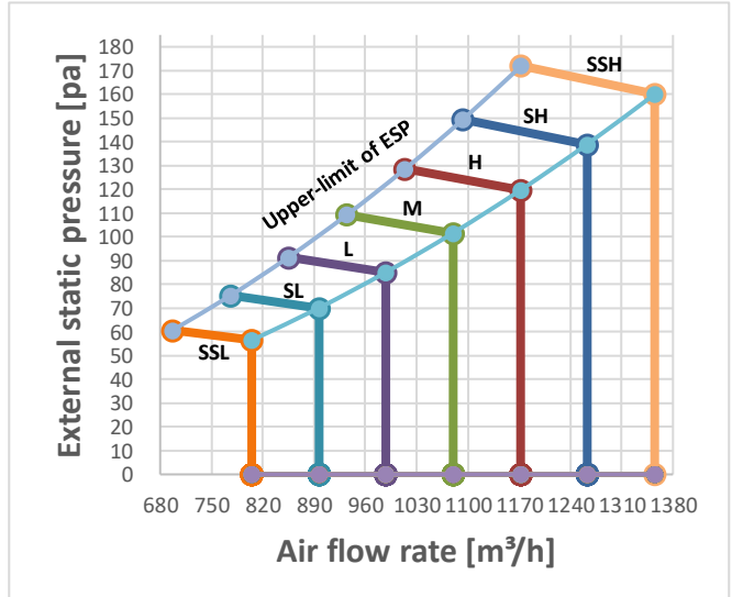
Figure 9.8: MIH80T2N18
