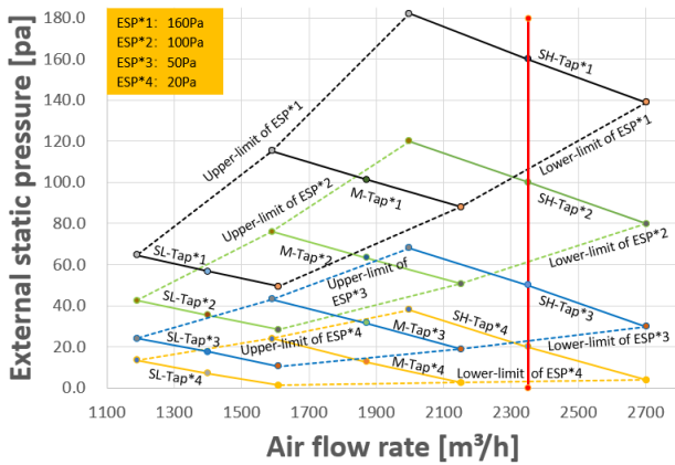
Figure 9.26: MIH160T2N18
