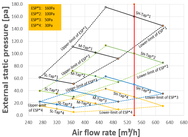
Figure 9.16: MIH28T2N18
