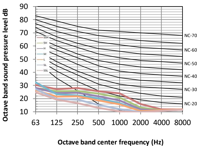
Figure 8.3: MIH15T2N18 octave band levels
