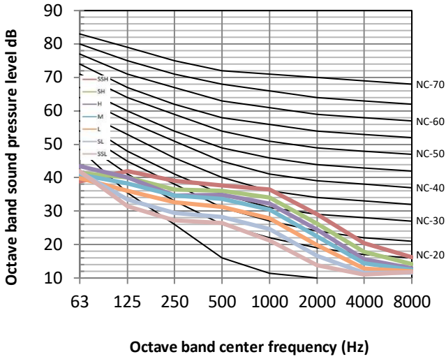
Figure 8.11: MIH90T2N18 octave band levels
