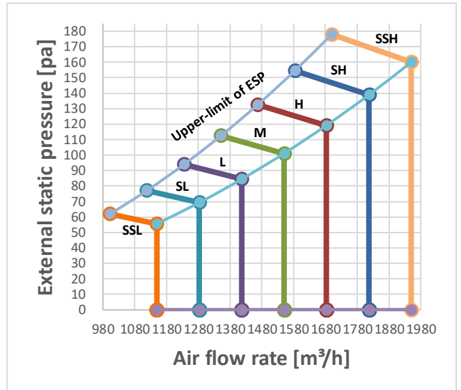
Figure 9.10: MIH112T2N18
