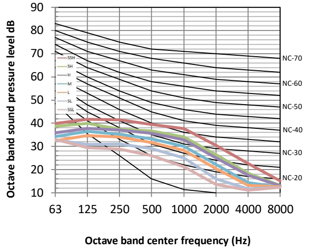
Figure 8.12: MIH112T2N18 octave band levels
