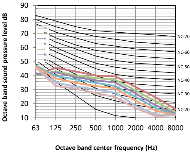
Figure 8.13: MIH125T2N18 octave band levels
