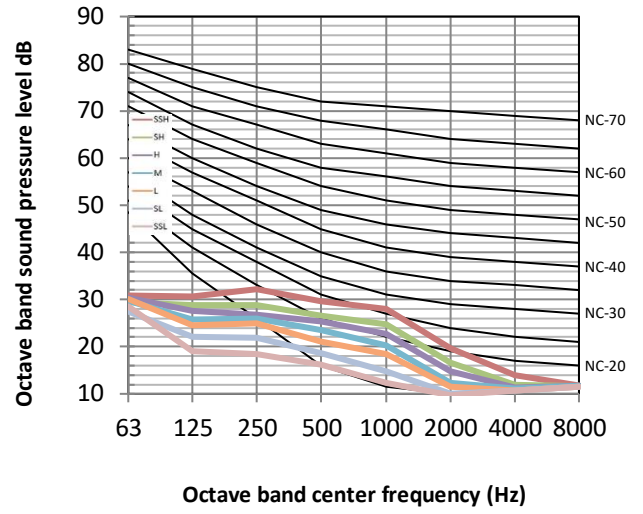
Figure 8.8: MIH56T2N18 octave band levels
