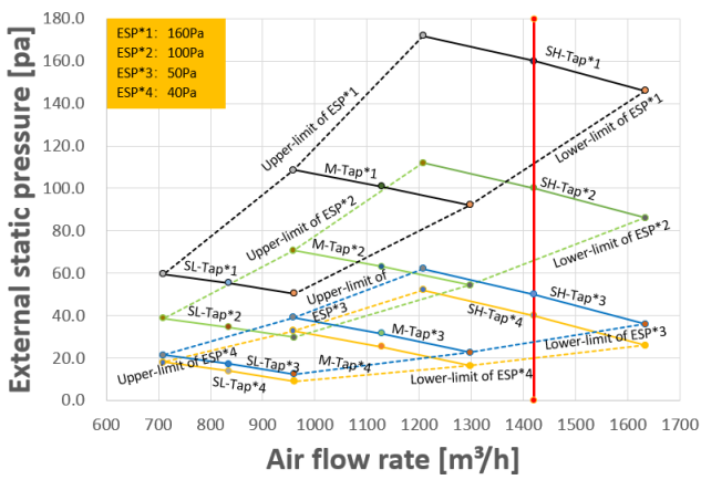
Figure 9.22: MIH90T2N18
