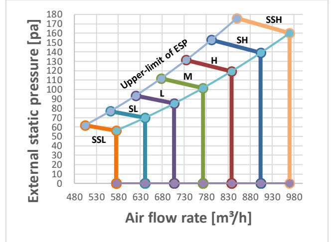
Figure 9.6: MIH56T2N18
