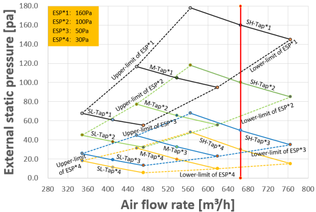
Figure 9.18: MIH45T2N18
