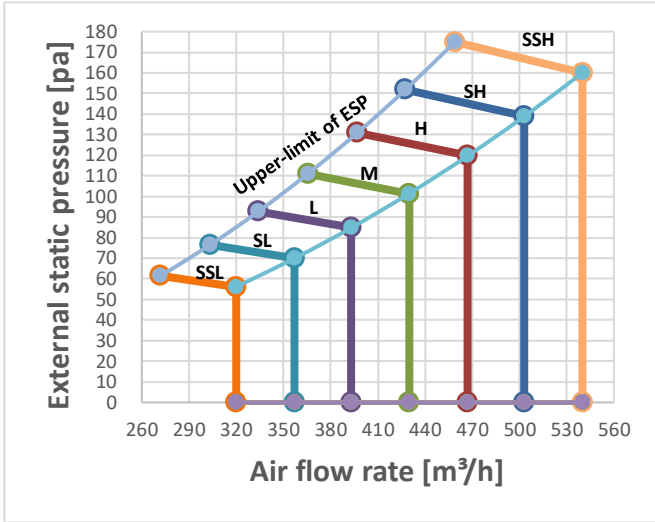
Figure 9.3: MIH28T2N18
