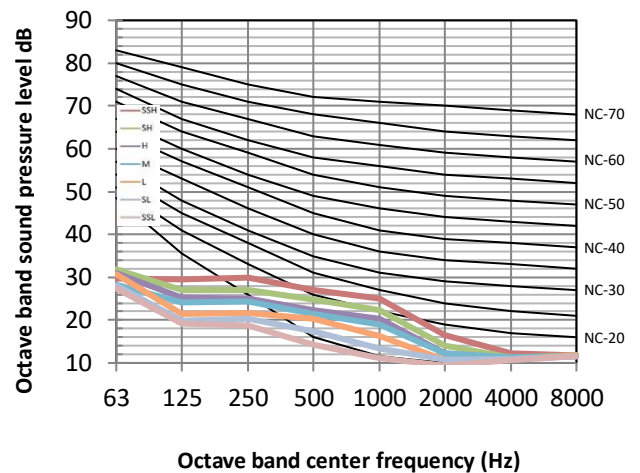
Figure 8.4: MIH22T2N18 octave band levels
