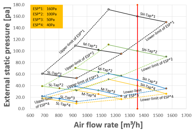
Figure 9.21: MIH80T2N18
