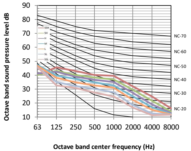
Figure 8.14: MIH140T2N18 octave band levels
