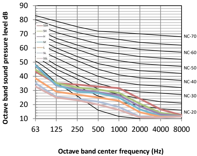
Figure 8.7: MIH45T2N18 octave band levels
