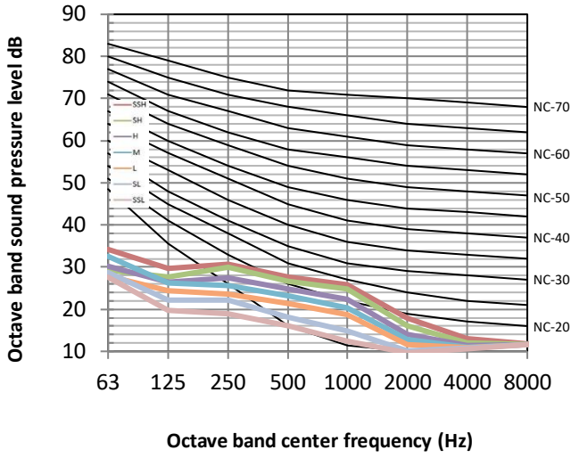
Figure 8.7: MIH45T2N18 octave band levels
