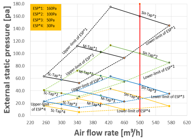
Figure 9.15: MIH22T2N18
