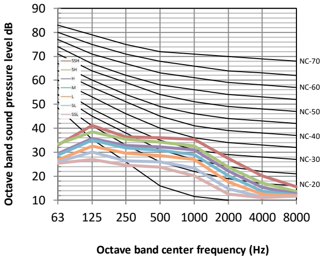
Figure 8.9: MIH71T2N18 octave band levels
