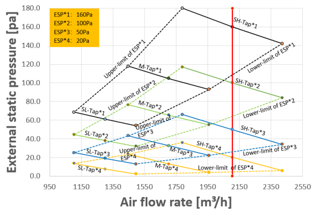
Figure 9.25: MIH140T2N18
