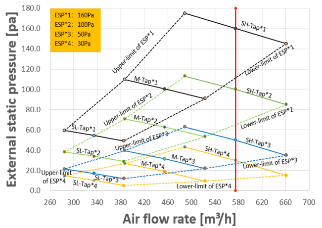
Figure 9.17: MIH36T2N18
