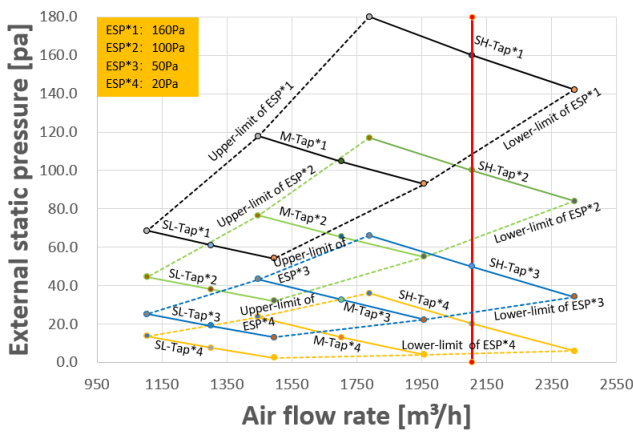
Figure 9.24: MIH125T2N18
