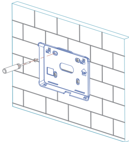
Figure 3 Attach back cover to wall
