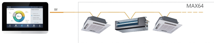
Figure 7(b) Connecting the centralized controller to the IDU (the first generation of AC/DC IDU)
