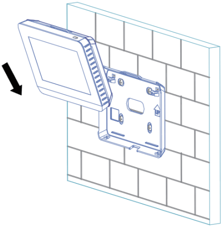
Figure 5 Insert controller into back cover
