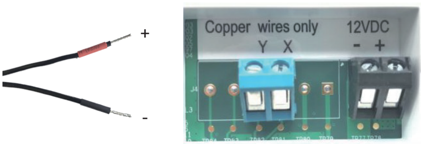
Figure 7(c) Adapter outlet terminal (12 VDC) shown in the left figure has a red positive pole and black negative pole. Connect it to the corresponding wiring terminal on the centralized controller back
