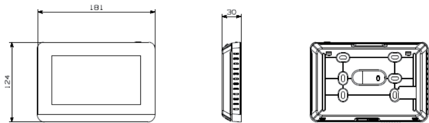
Figure 1 Front view and back view of the centralized controller
