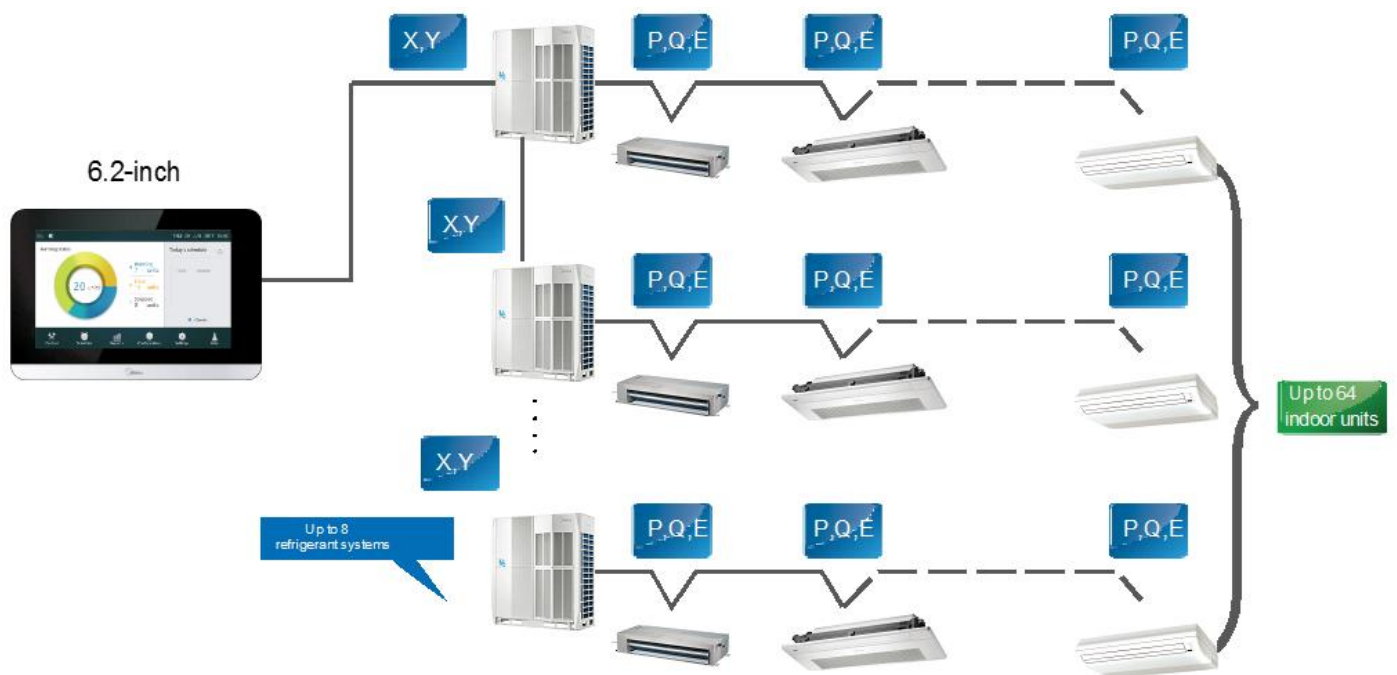
Figure 7(a) Connecting the central controller to the ODU
