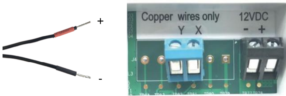
Figure 7(c) Adapter outlet terminal (12 VDC) shown in the left figure has a red positive pole and black negative pole. Connect it to the corresponding wiring terminal on the central controller back
