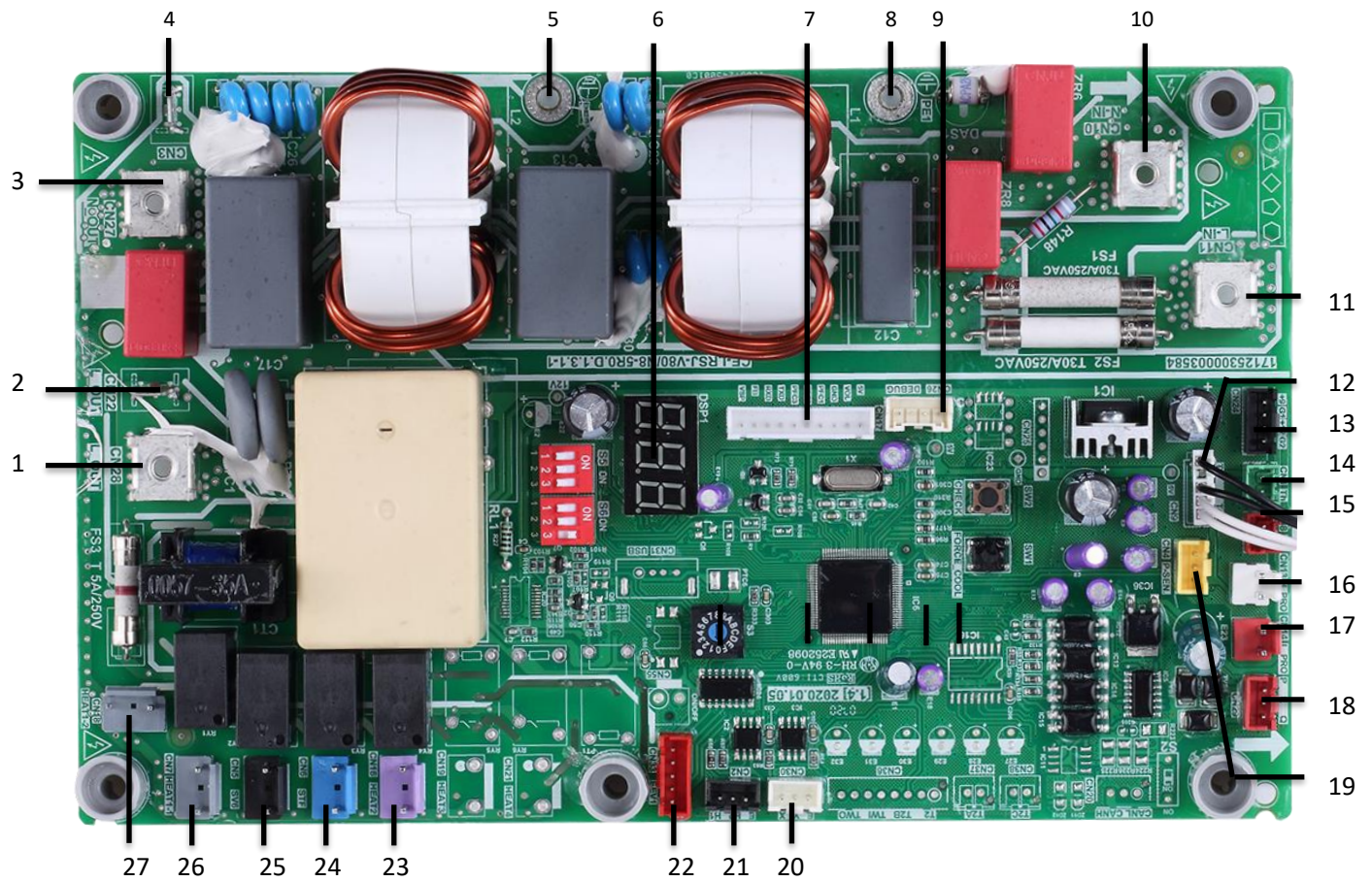
Figure 4-2.4: MHC-V12( 14, 16)W/D2N8-B outdoor unit main PCB for refrigerant system 1
