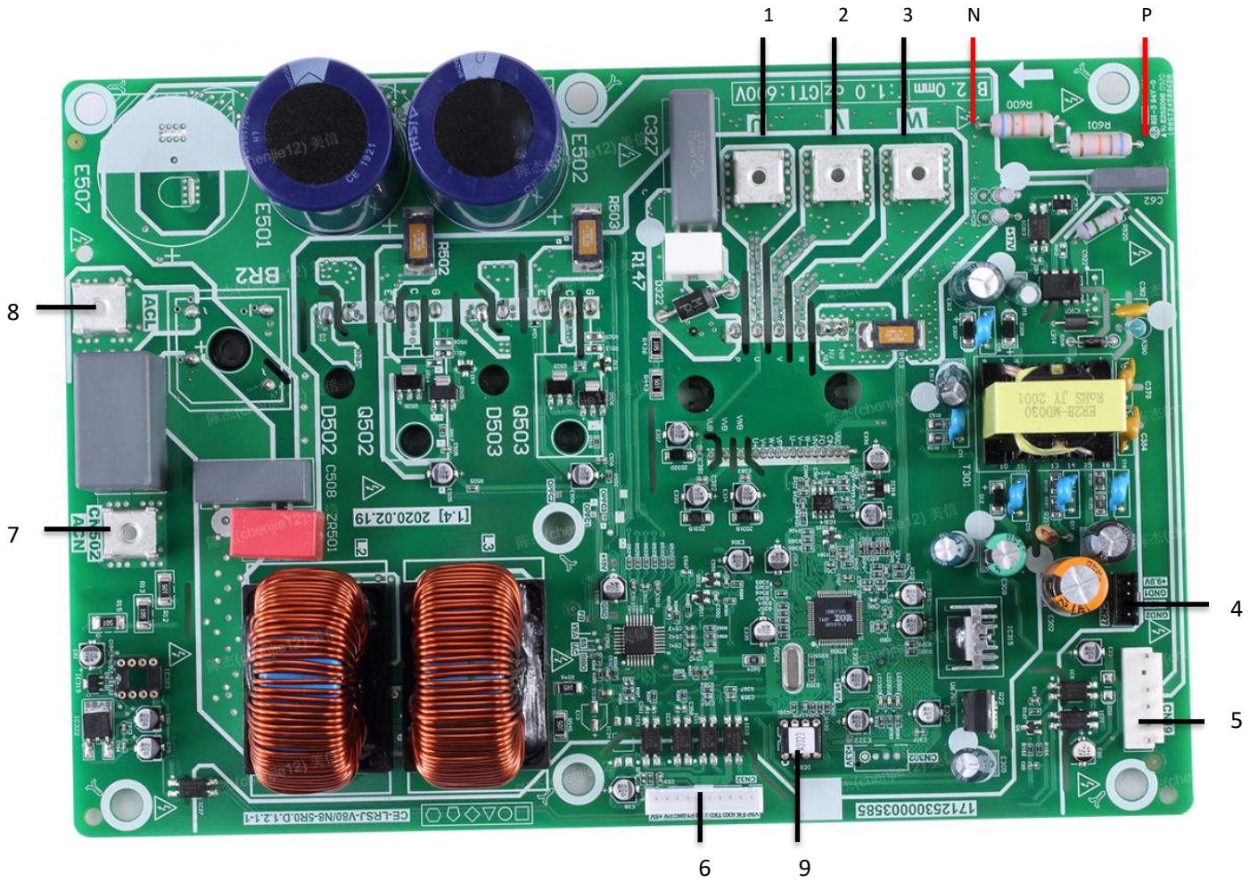
Figure 4-2.3: MHC-V4(6)W/D2N8-B outdoor unit inverter module
