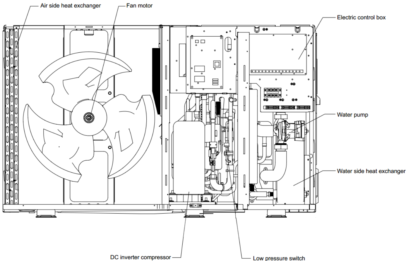
Figure 2-1.5: MHC-V12( 14, 16)W/D2N8-B, MHC-V12(14, 16)W/D2RN8-B front view
