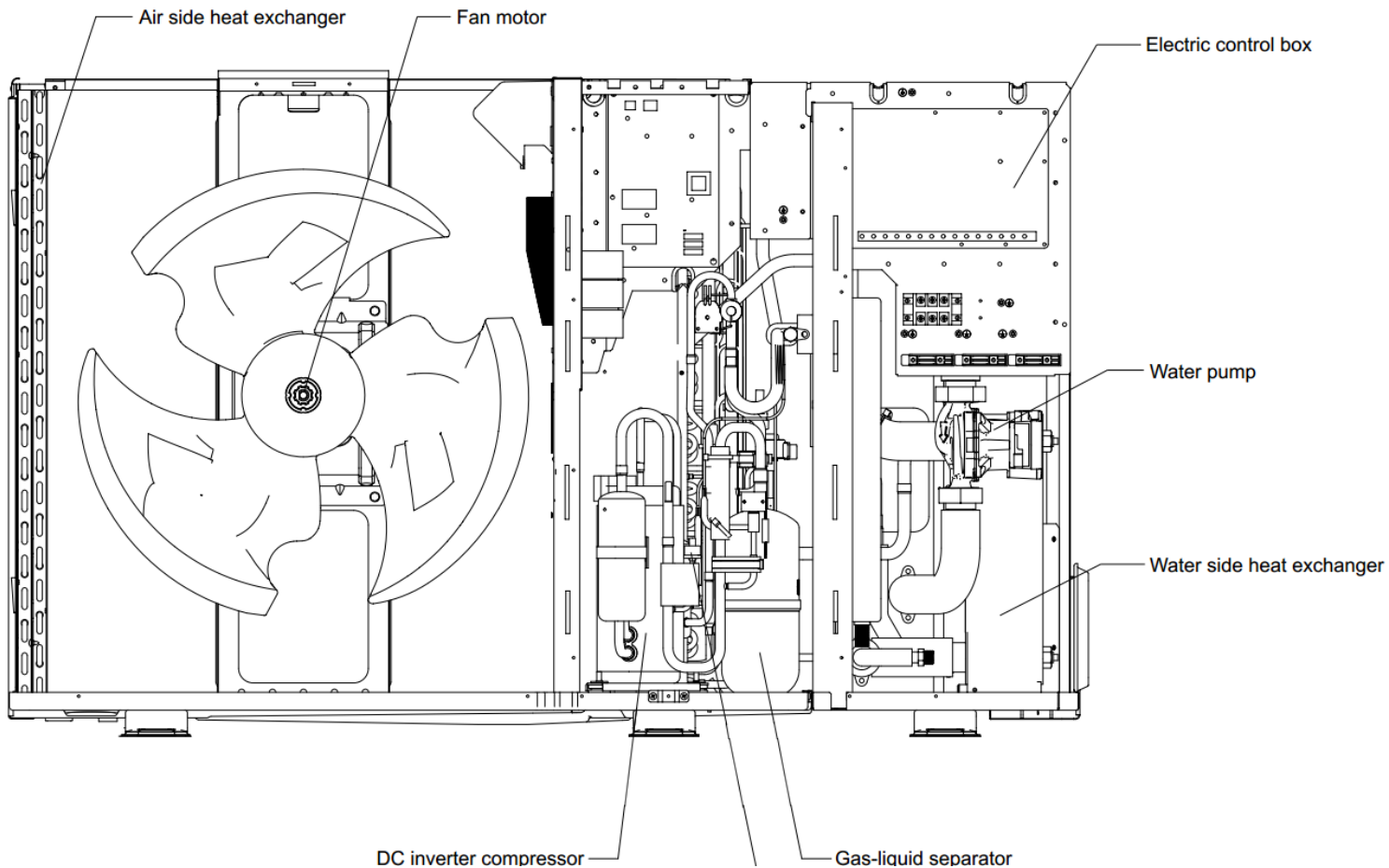
Figure 2-1.2: MHC-V8(10)W/D2N8-B front view
