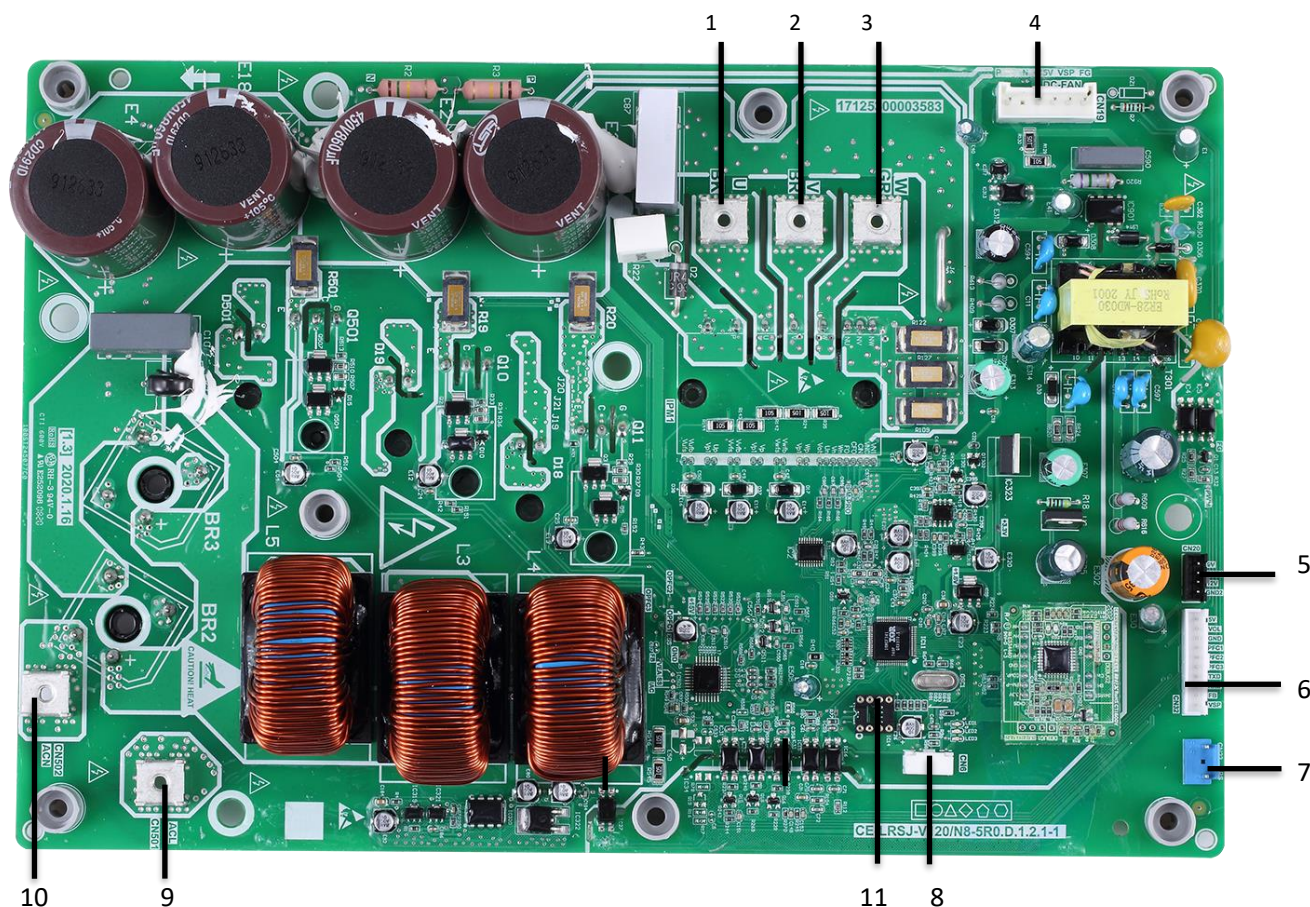
Figure 4-2.5: MHC-V12( 14, 16)W/D2N8-B outdoor unit inverter module
