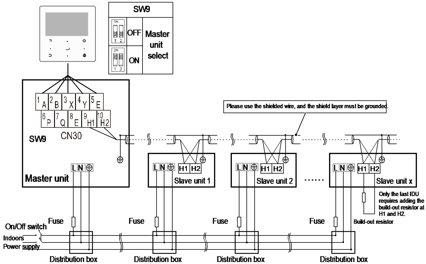
Figure 4-3.4 Combination system diagram for single phase 4~16kW models
