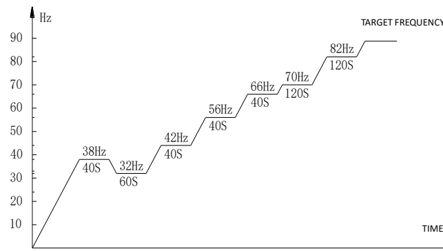
Figure 3-3.1: 4-6kW to 12-16kW Compressor startup program 1,2 when ambient temperature is above 3°C
