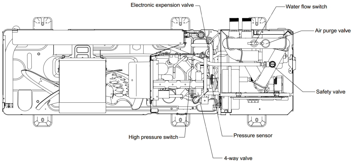
Figure 2-1.2: MHC-V8(10)W/D2N8-B front view
