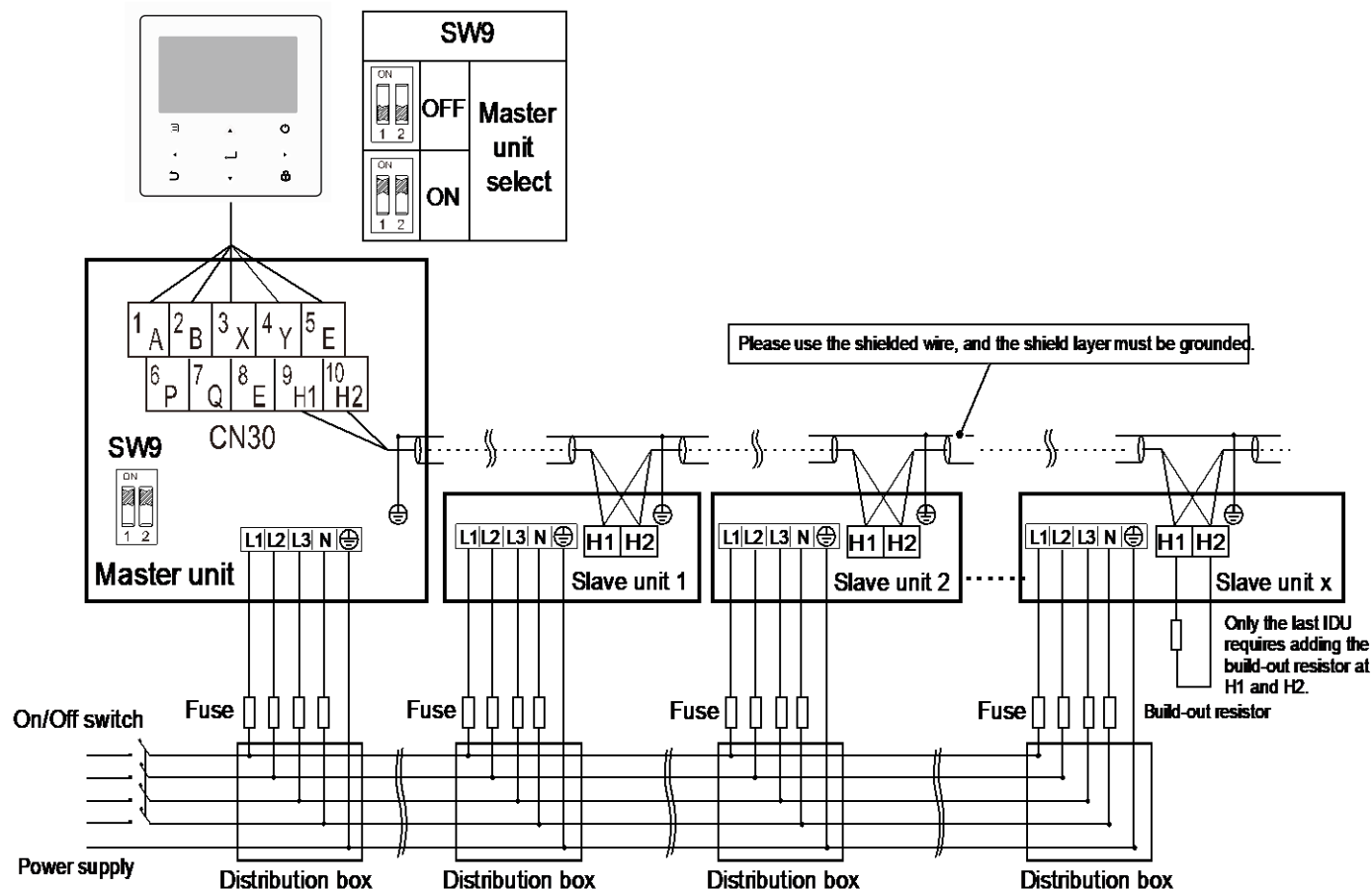
Figure 4-3.5 Combination system diagram for three phase 12~16kW models
