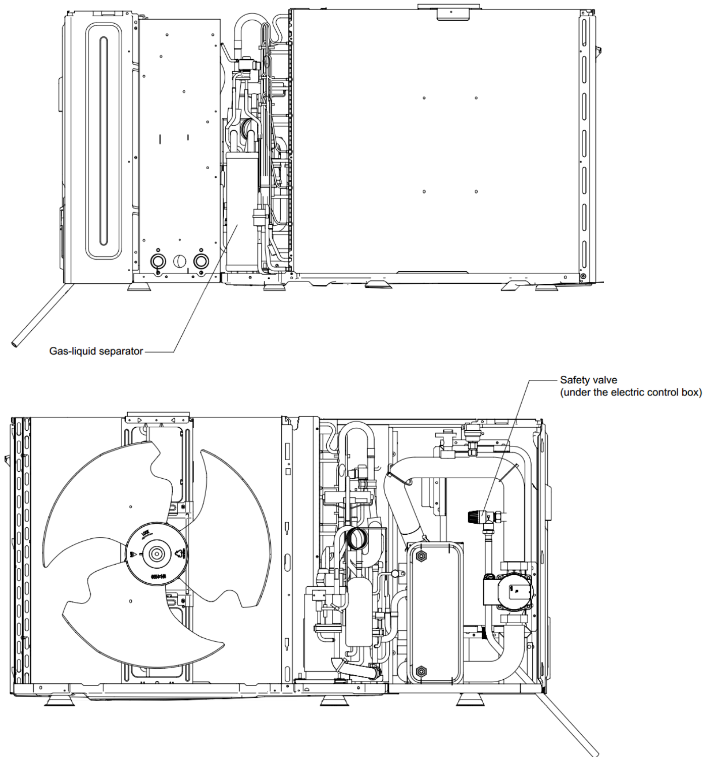
Figure 2-1.3: MHC-V4(6)W/D2N8-B
