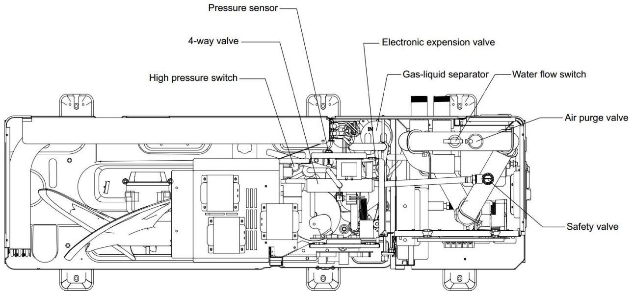
Figure 2-1.5: MHC-V12( 14, 16)W/D2N8-B, MHC-V12(14, 16)W/D2RN8-B front view
