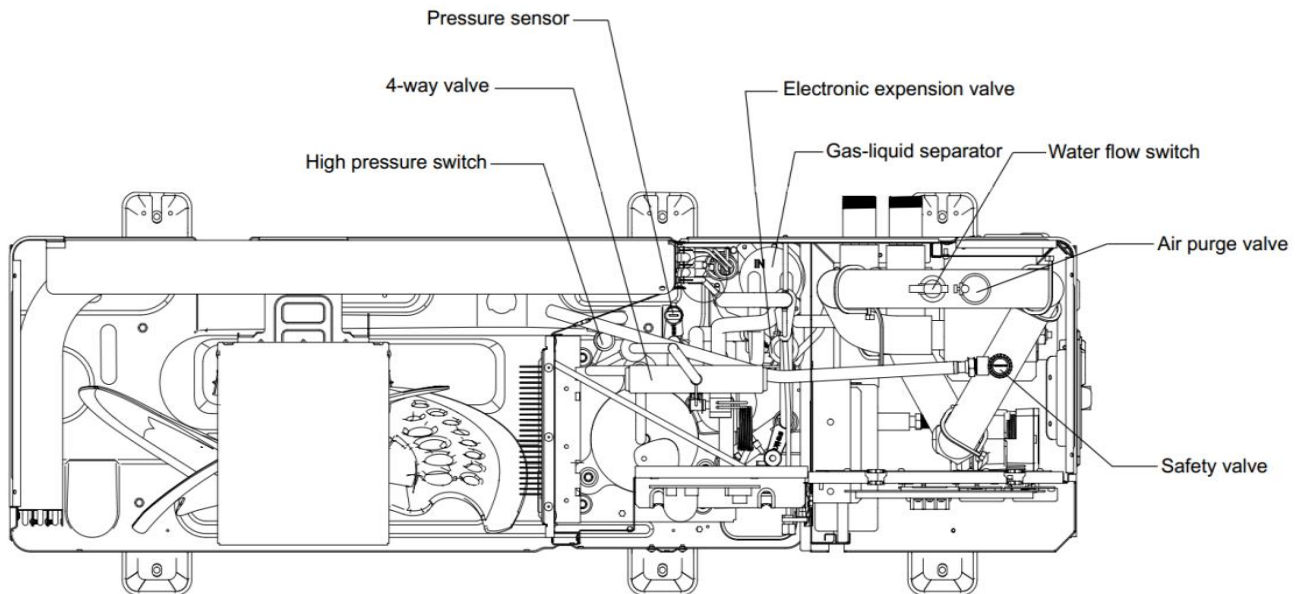
Figure 2-1.4: MHC-V12(14, 16)W/D2N8-B top view
