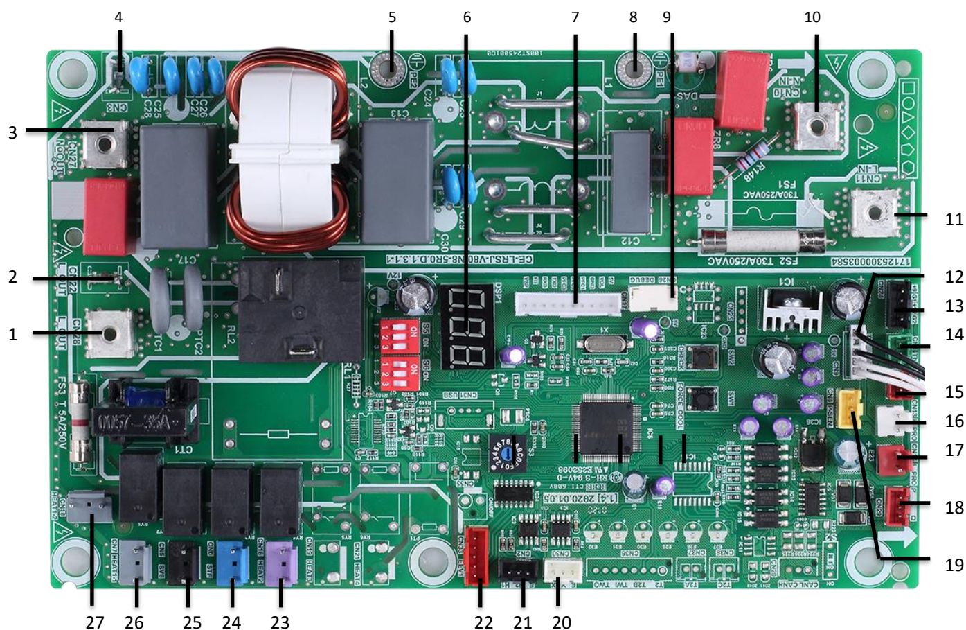
Figure 4-2.2: MHC-V4(6,8,10)W/D2N8-B outdoor unit main PCB for refrigerant system
