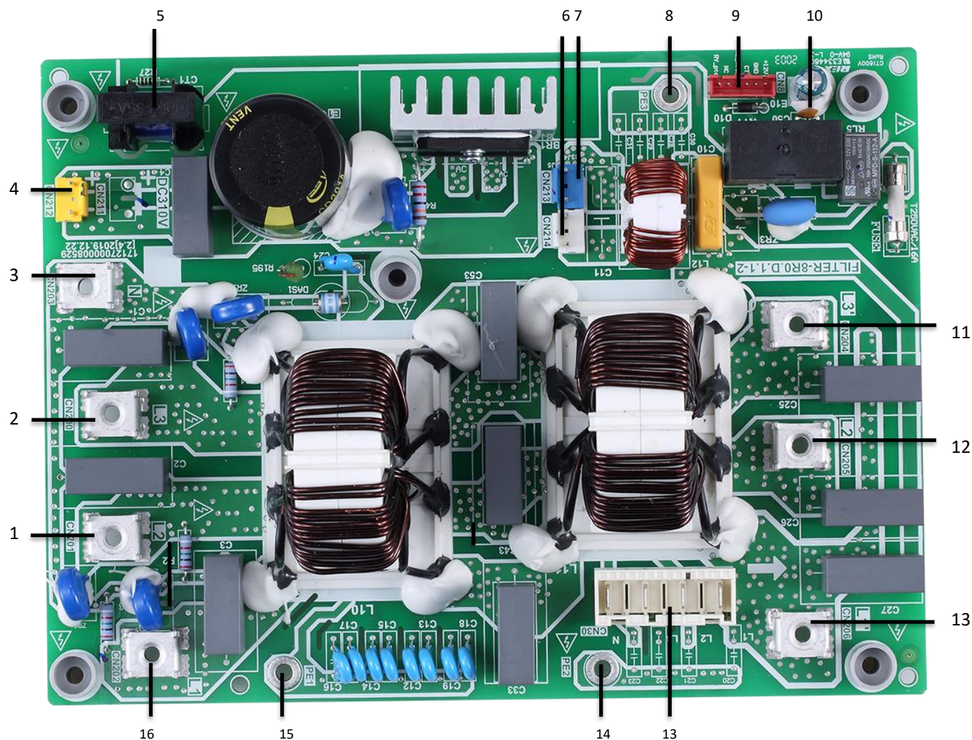
Figure 4-2.8: MHC-V12(14, 16)W/D2RN8-B outdoor unit filter board
