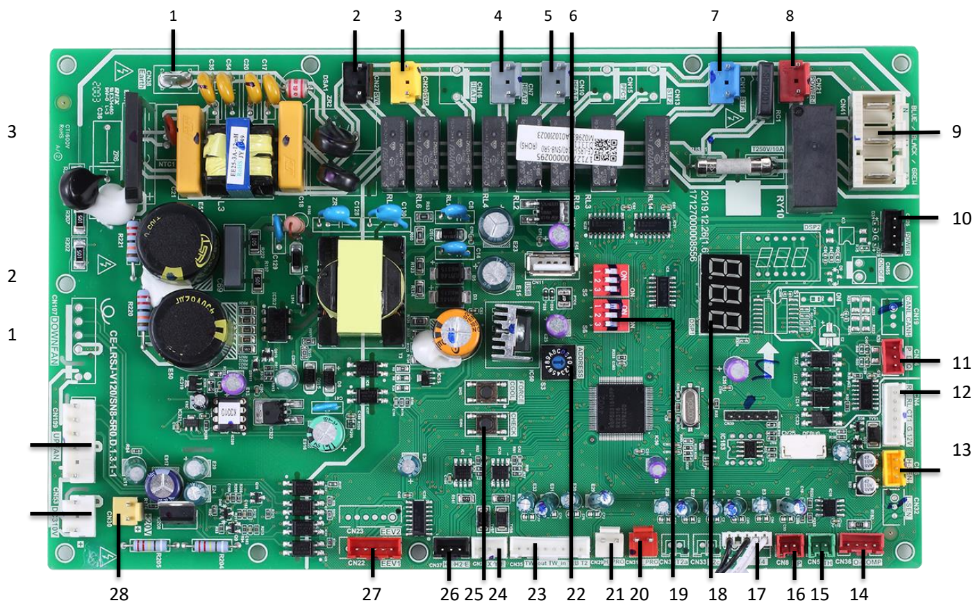
Figure 4-2.6: MHC-V12(14, 16)W/D2RN8-B outdoor unit main PCB for refrigerant system 1
