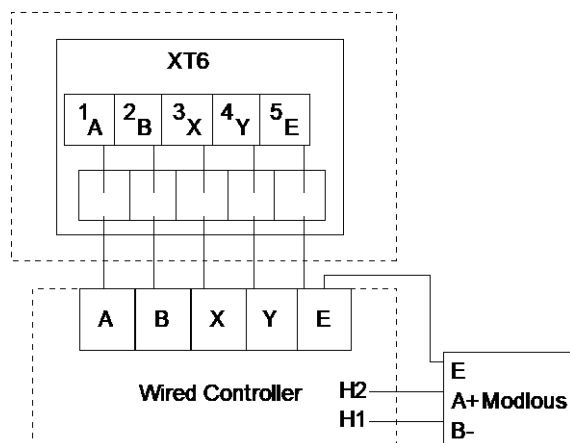
Figure 4-2.11: Wiring
