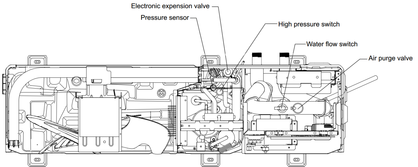
Figure 2-1.2: MHC-V4(6)W/D2N8-B front view
