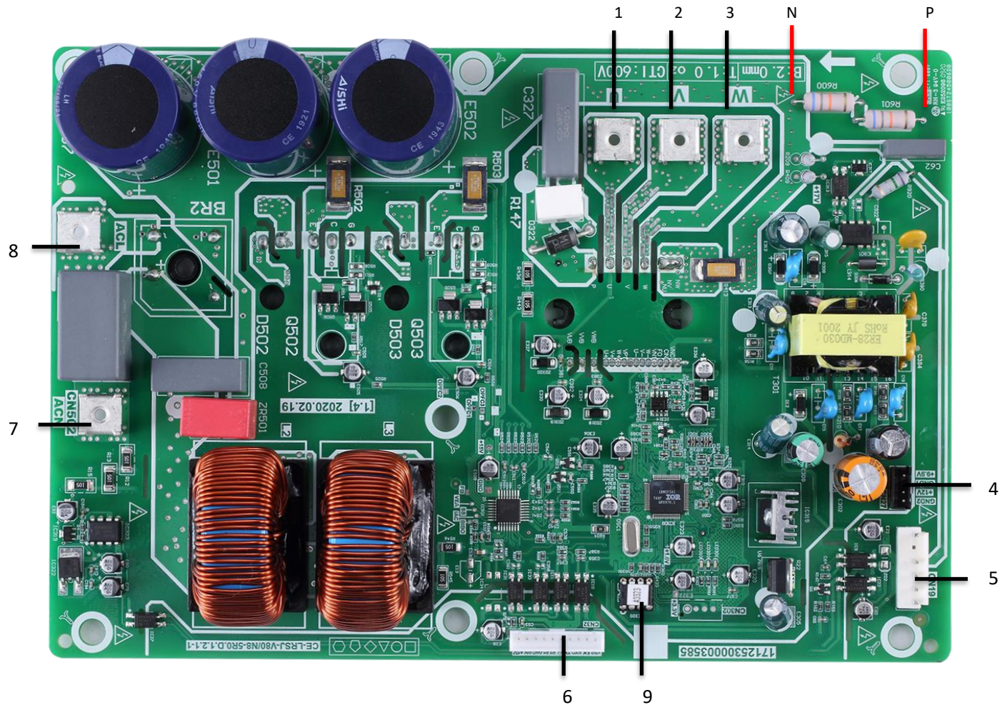
Figure 4-2.3: MHC-V8(10)W/D2N8-B outdoor unit inverter module
