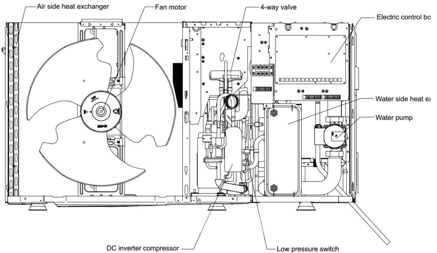
Figure 2-1.2: MHC-V4(6)W/D2N8-B front view
