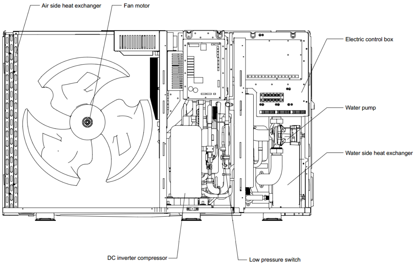
Figure 2-1.5: MHC-V12( 14, 16)W/D2N8-B, MHC-V12(14, 16)W/D2RN8-B front view
