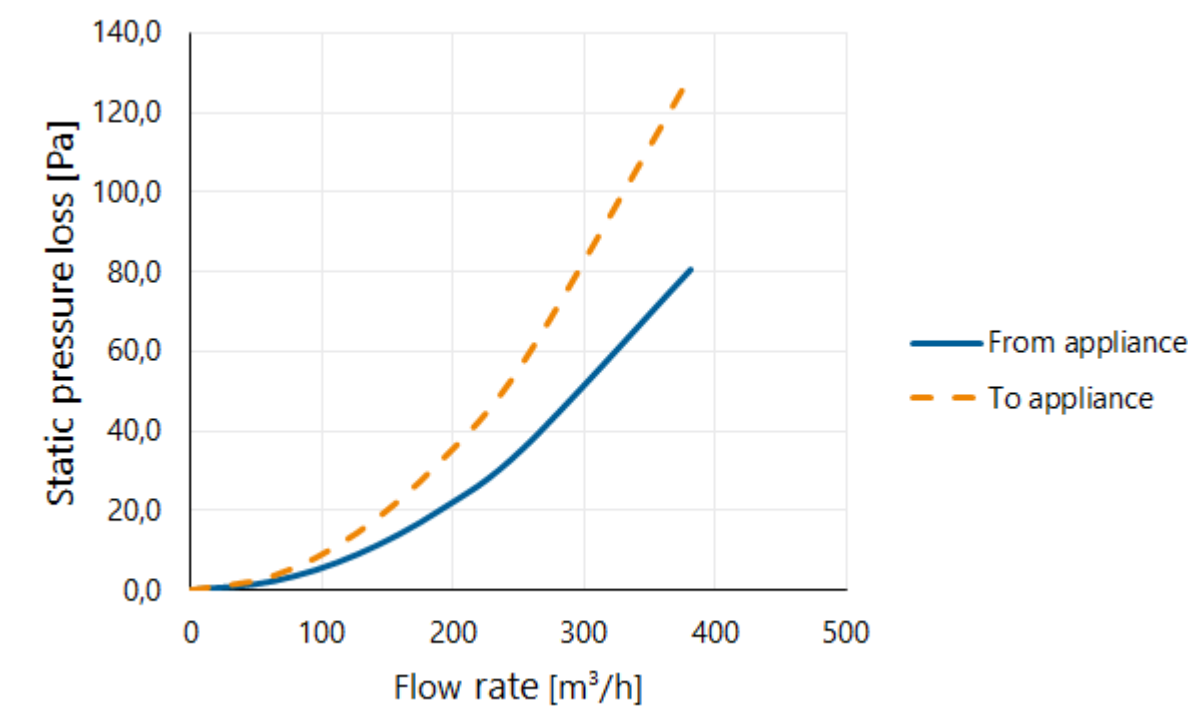
Pressure loss
