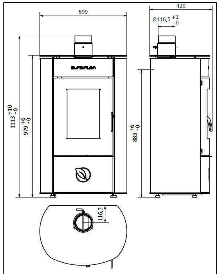
Image 2 Dimensions
