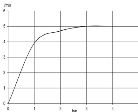
Diagrama debit
