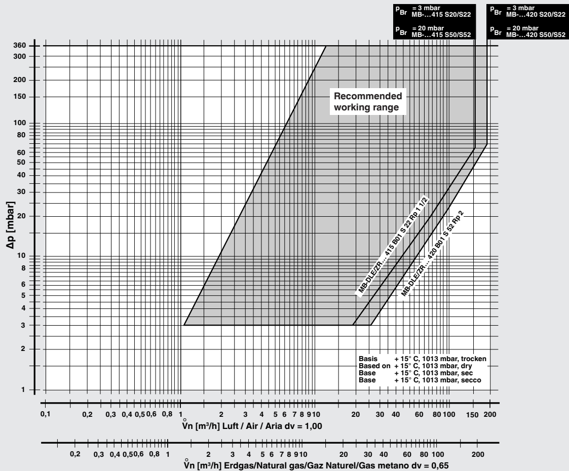
Volumetric flow pressure loss characteristics in regulated state with microfilter
