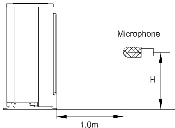
Outdoor Unit
