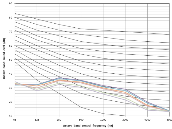
Figure 10.15:MIH80F4N18,MIH80F5N18 octave band levels
