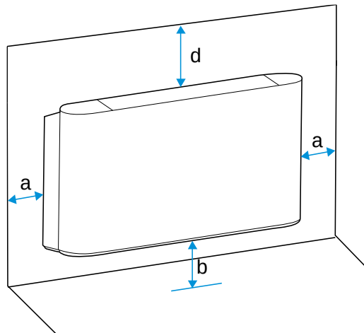
Figure 3.1: F4 series (air inlet from front) Exposed Floor Standing space requirements (unit: mm)
