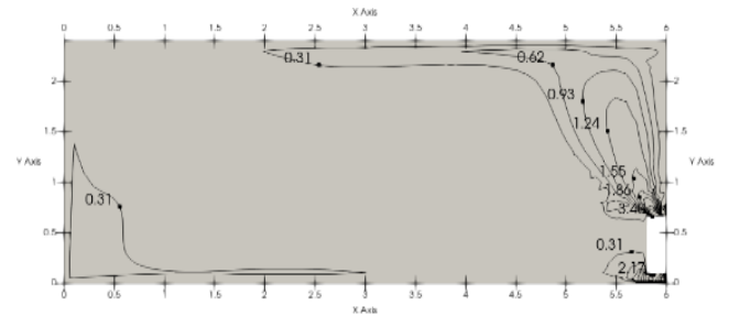
Figure 11.14: MIH80 F3(4,5)N18 heating at 300S
