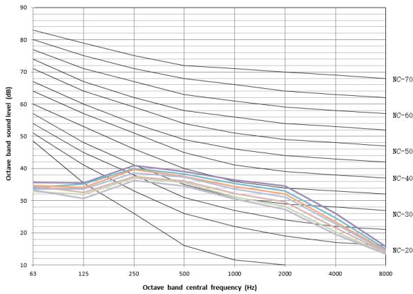
Figure 10.15:MIH80F4N18,MIH80F5N18 octave band levels
