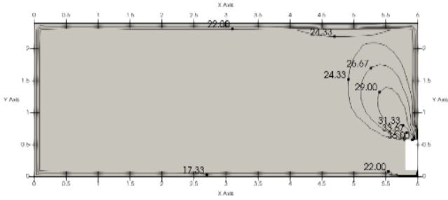
Figure 11.16: MIH22 F3 (4,5)N18 heating at 300S
