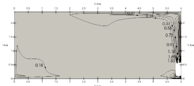
Figure 11.5: MIH36 F3(4,5)N18 cooling at 300S
