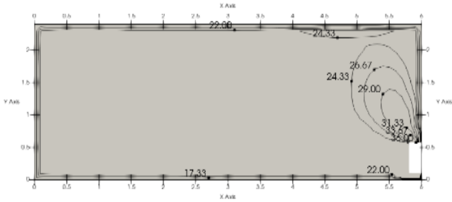
Figure 11.20: MIH36 F3 (4,5)N18 heating at 300S
