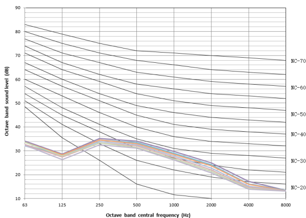
Figure 10.2: MIH22F3N18 octave band levels
