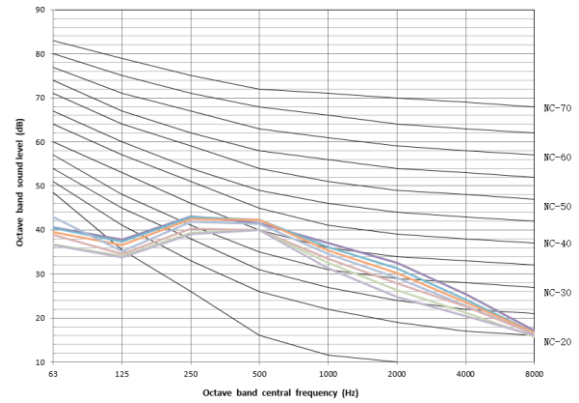
Figure 10.7: MIH71F3N18 octave band levels
