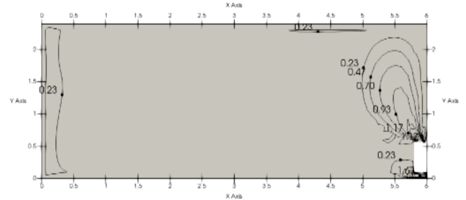
Figure 11.10: MIH56 F3(4,5)N18 heating at 300S
