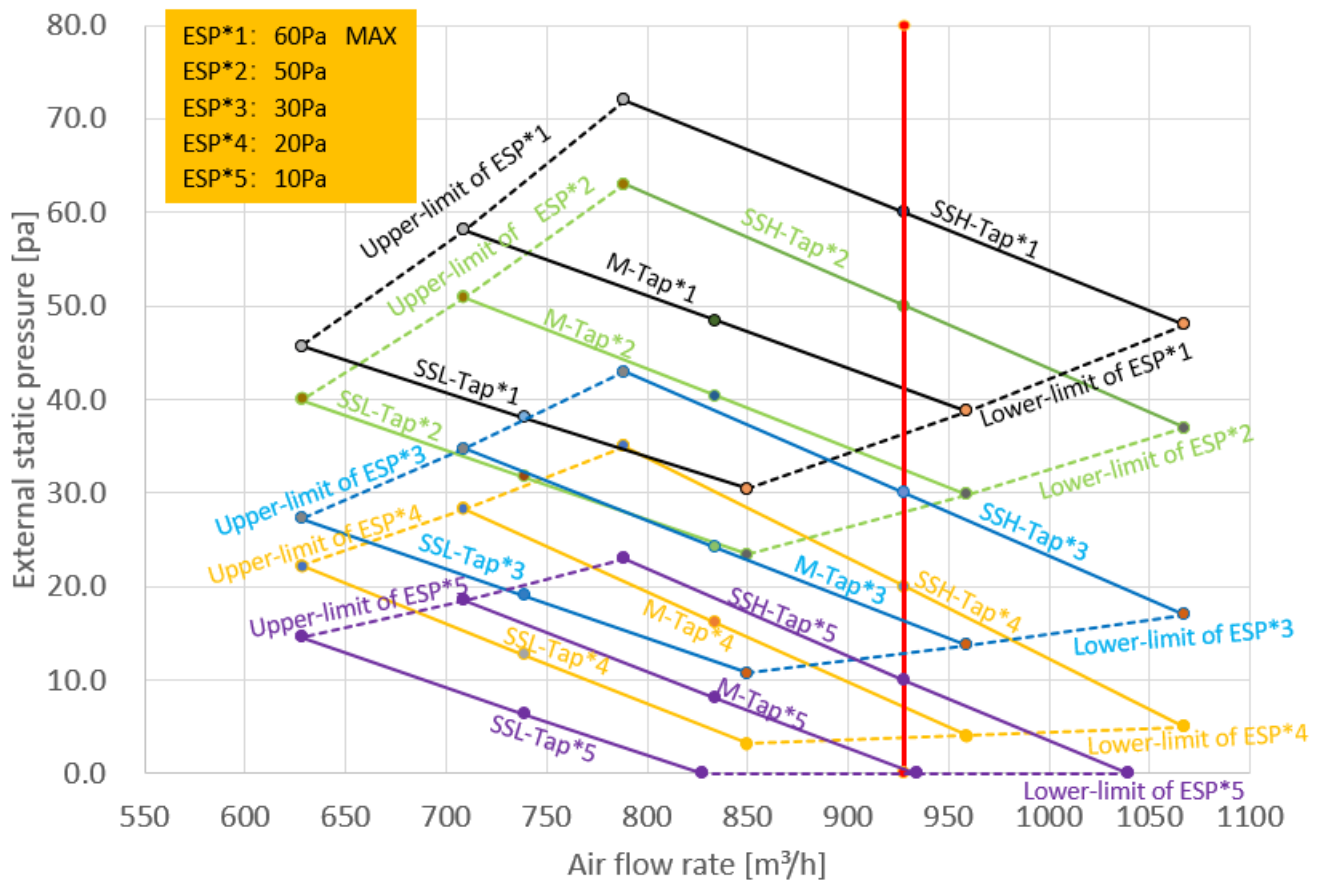
Figure 9.6: MIH71F3N18 fan performance
