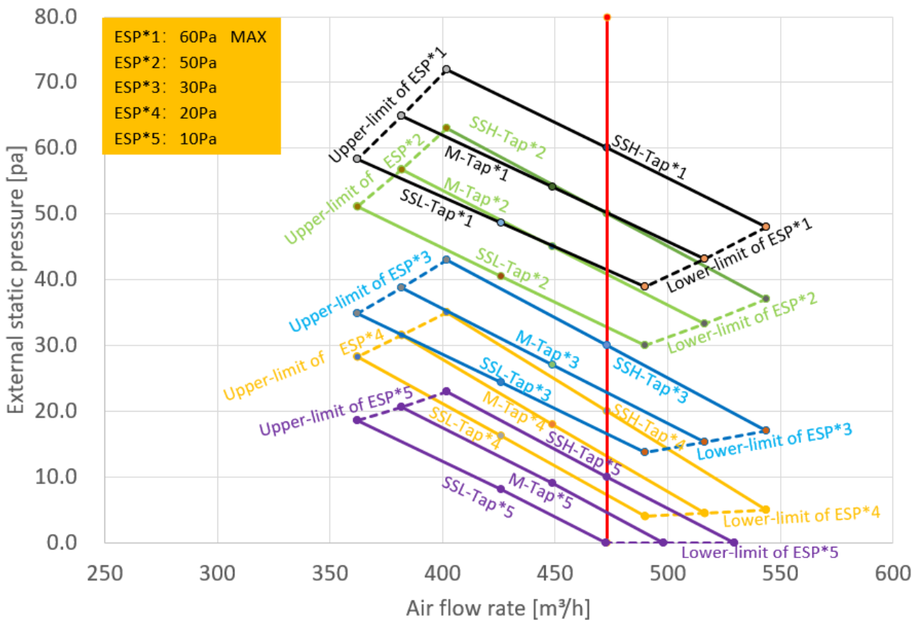
Figure 9.2: MIH28F3N18 fan performance
