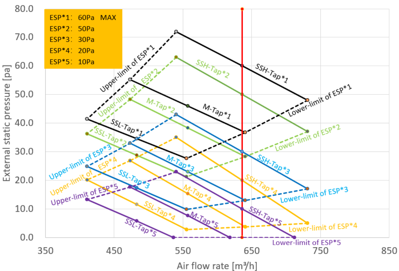
Figure 9.4: MIH45F3N18 fan performance
