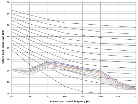
Figure 10.13:MIH56F4N18,MIH56F5N18 octave band levels
