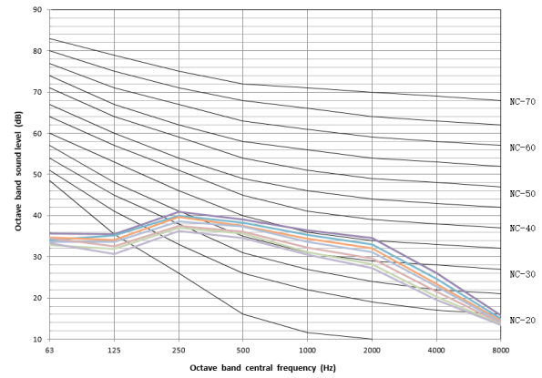
Figure 10.14:MIH71F4N18,MIH71F5N18 octave band levels
