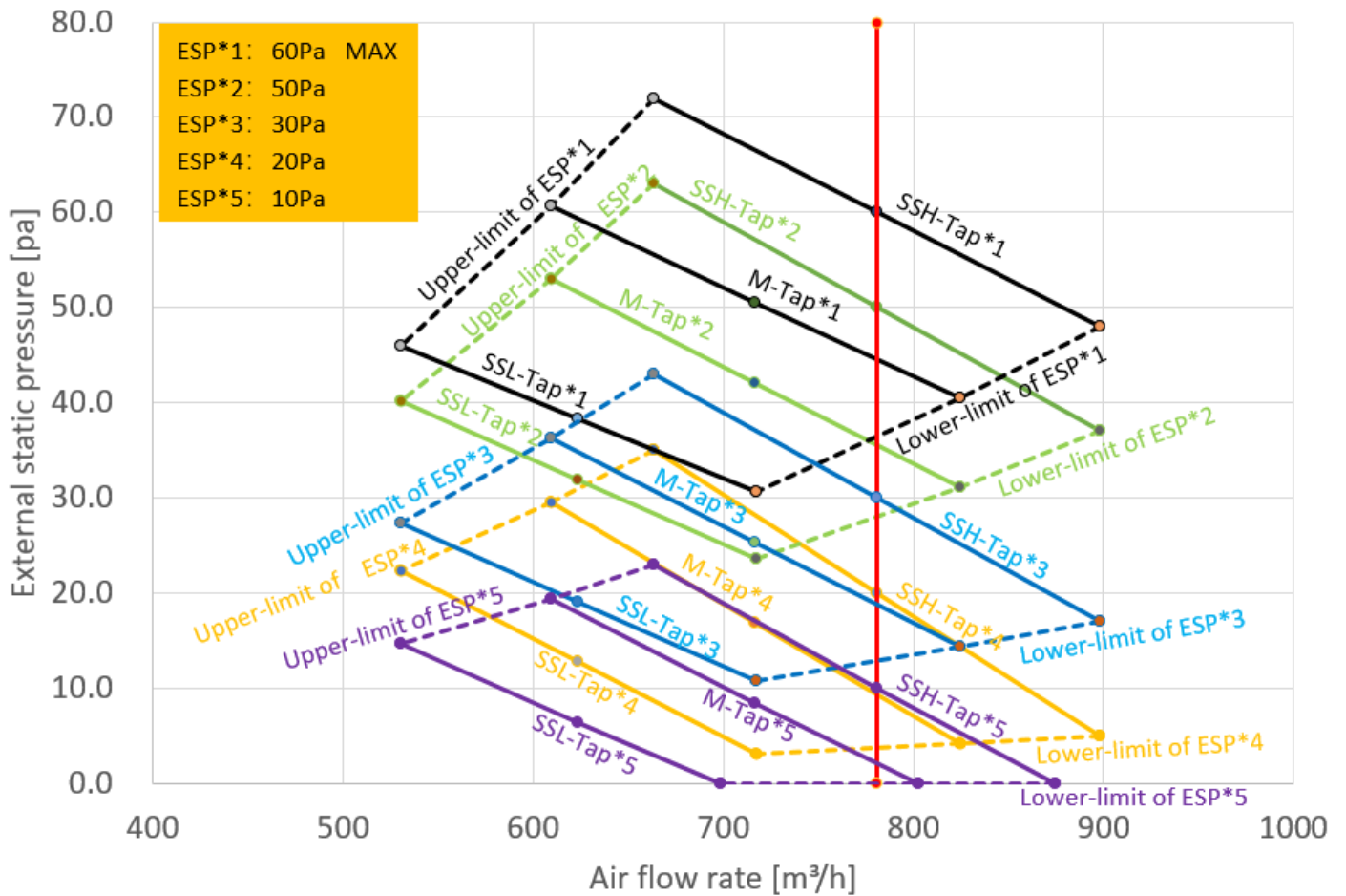
Figure 9.6: MIH71F3N18 fan performance
