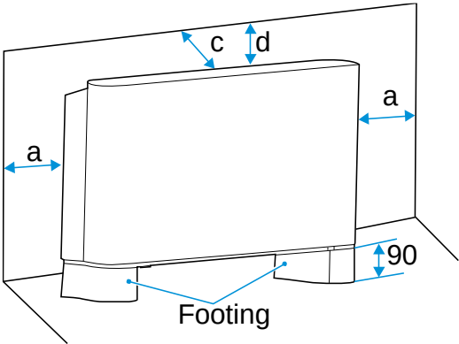
Figure 3.2: F5 series (air inlet from bottom) Exposed Floor Standing space requirements (unit: mm)
