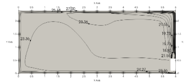
Figure 11.19: MIH36 F3 (4,5)N18 cooling at 300S
