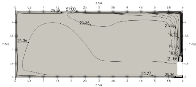
Figure 11.15: MIH22 F3 (4,5)N18 cooling at 300S
