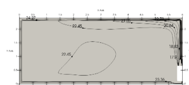
Figure 11.23: MIH56 F3 (4,5)N18 cooling at 300S
