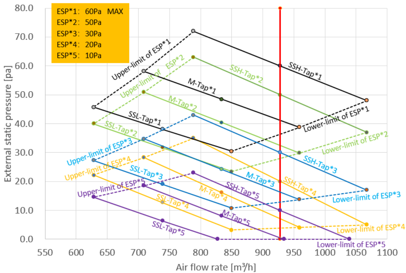
Figure 9.7: MIH80F3N18 fan performance
