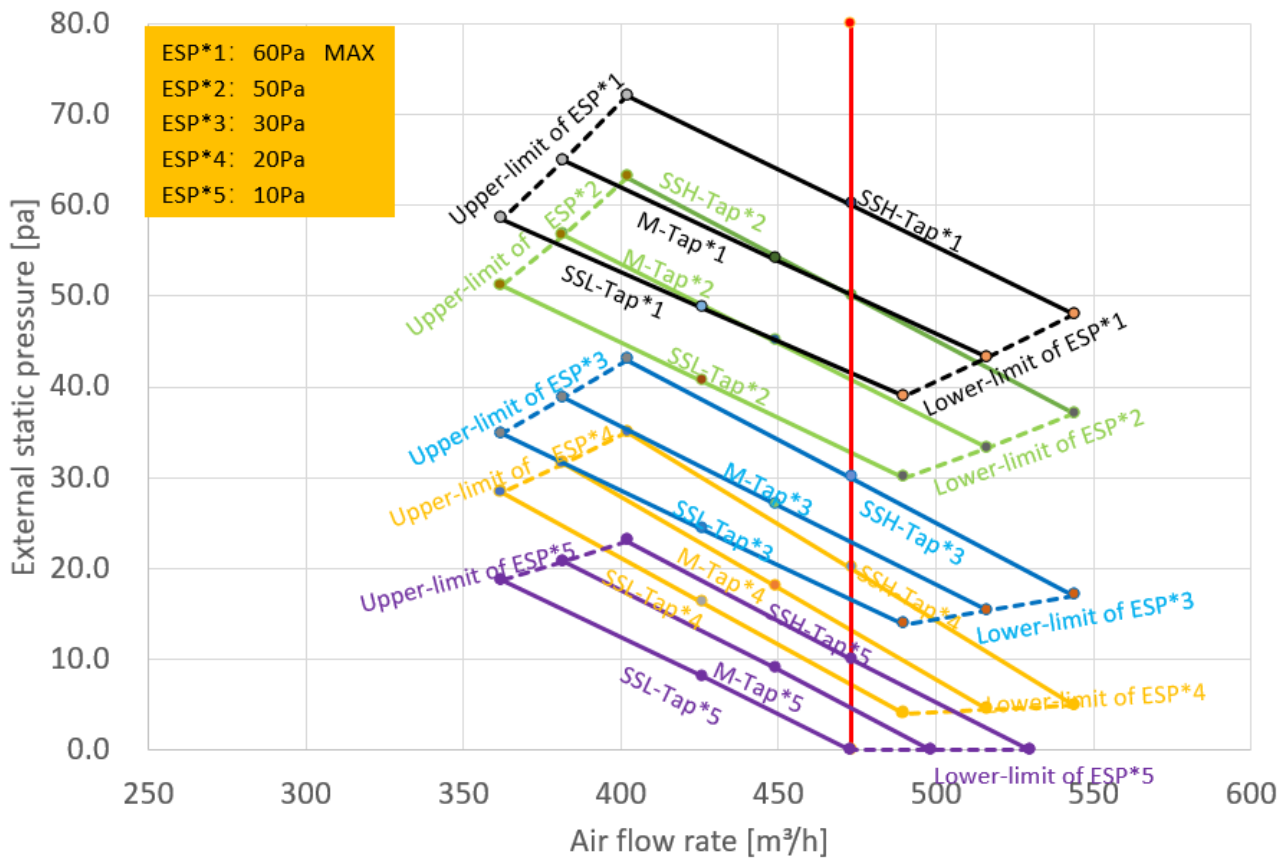
Figure 9.1: MIH22F3N18 fan performance
