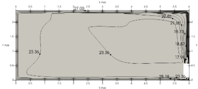
Figure 11.21: MIH45 F3 (4,5)N18 cooling at 300S
