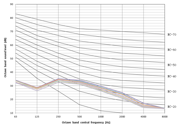
Figure 10.3: MIH28F3N18 octave band levels
