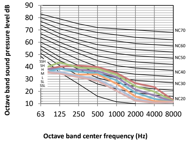
Figure 8.3: MIH56Q4CN18 octave band levels
