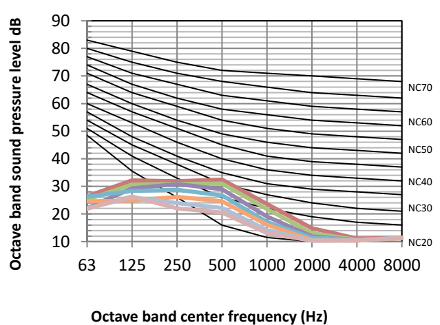
Figure 8.3: MIH36Q4CN18 octave band levels
