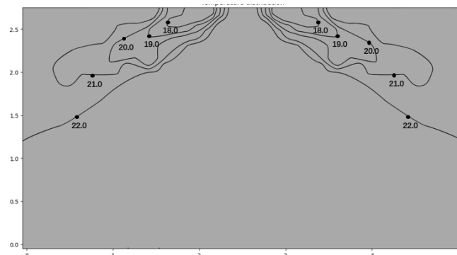
Figure 9.1: MIH15Q4CN18 cooling at 300s
