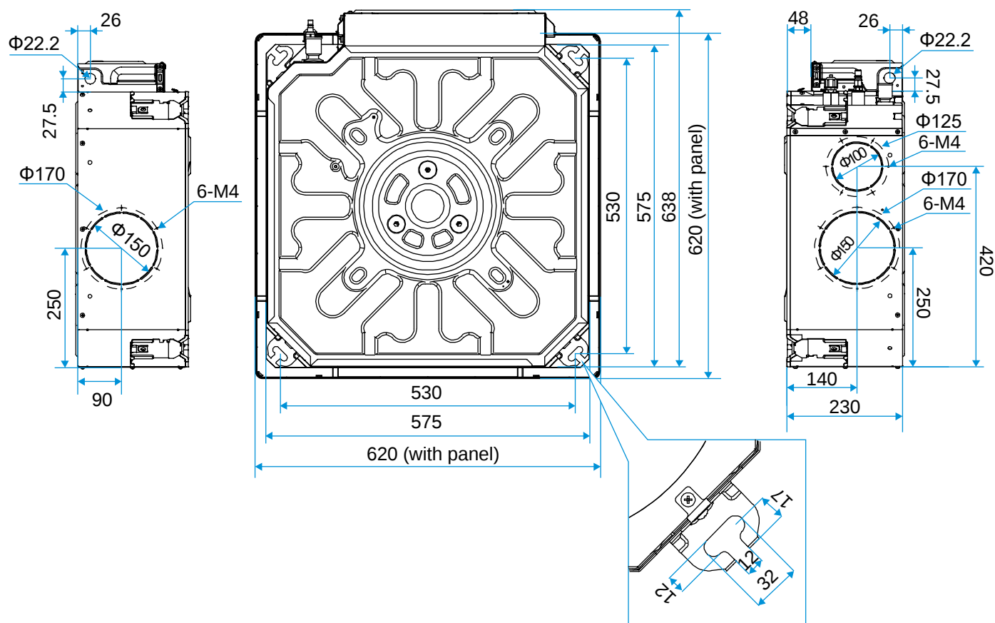
Figure 2.1: Compact Four-way Cassette dimensions (unit: mm)
