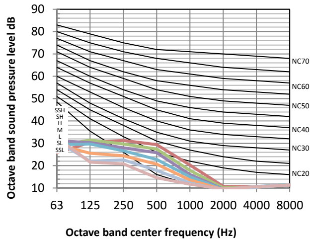
Figure 8.3: MIH36Q4CN18 octave band levels
