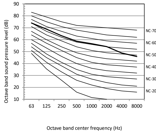
Figure 2-10.3: 16HP octave band level
