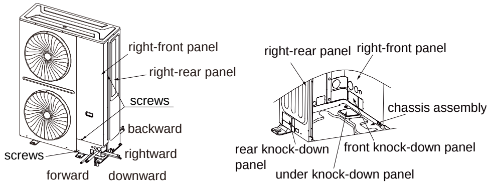
Figure 3-5.13: Direction of refrigerant pipe connection
