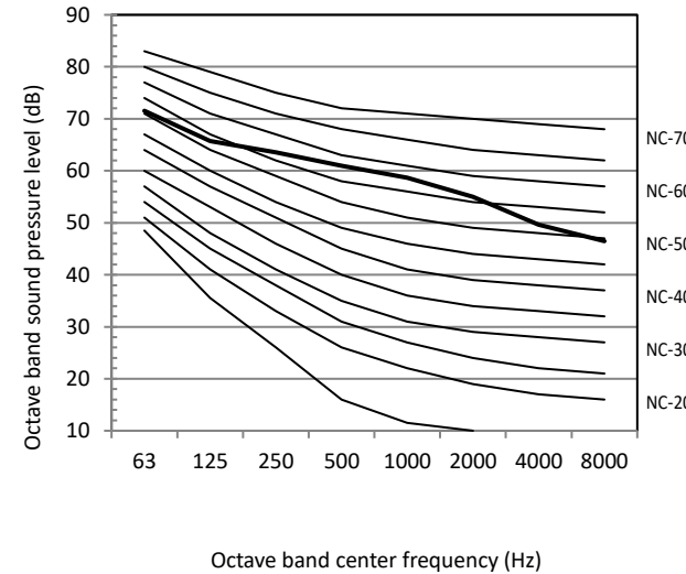
Figure 2-10.5: 20HP octave band level
