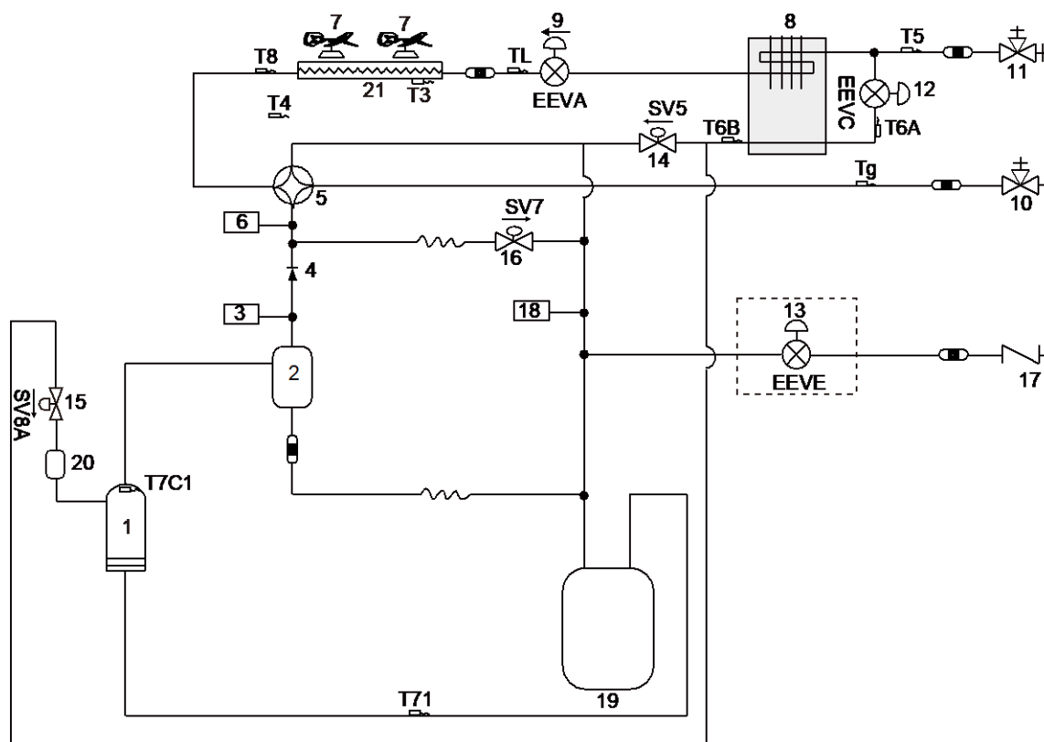
Figure 2-4.1: 14HP piping diagram
