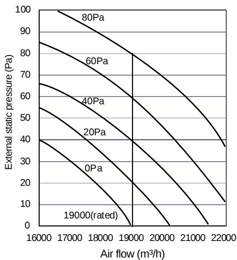
Figure 3-3.6: 22HP units fan performance
