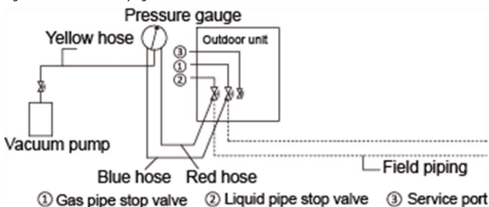
Figure 3-5.15: Vacuum drying
