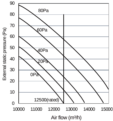
Figure 3-3.4: 18HP units fan performance
