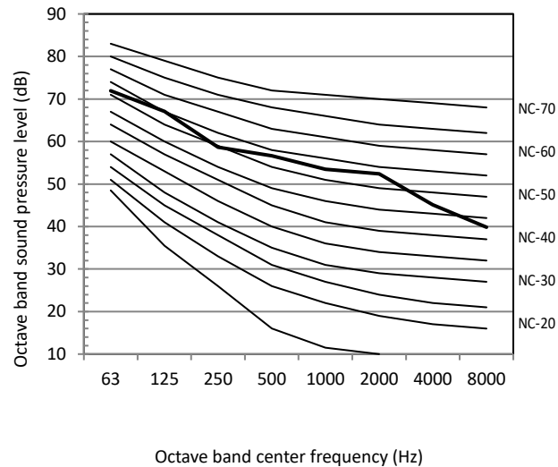
Figure 2-10.2: 14HP octave band level
