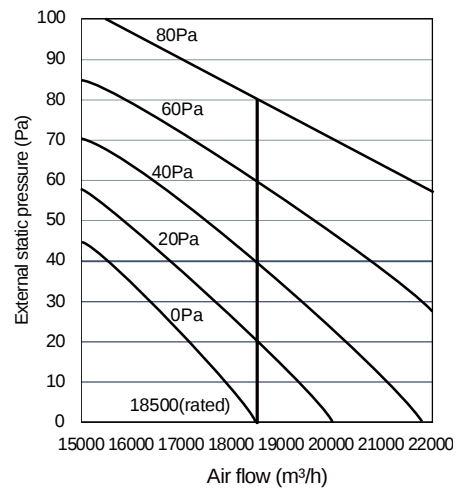
Figure 3-3.5: 20HP units fan performance
