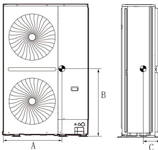
Figure 3-2.5: 14-24HP Center of gravity
