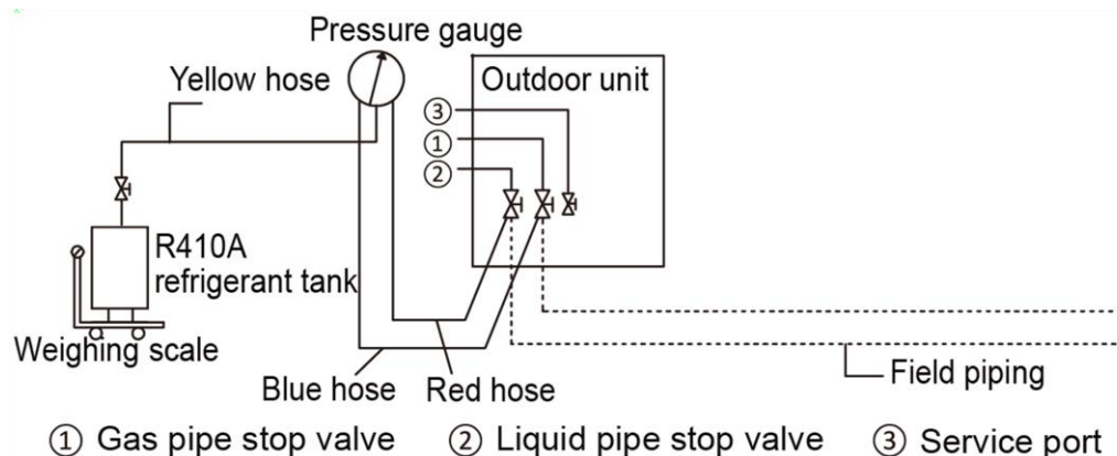
Figure 3-8.1: Charging refrigerant
