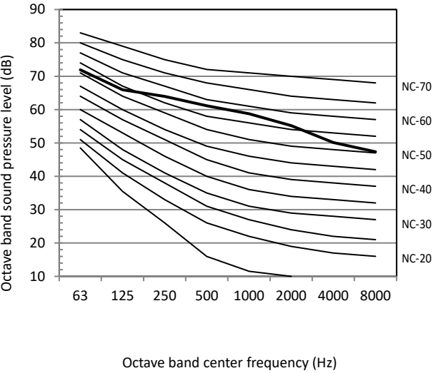
Figure 2-10.6: 22HP octave band level
