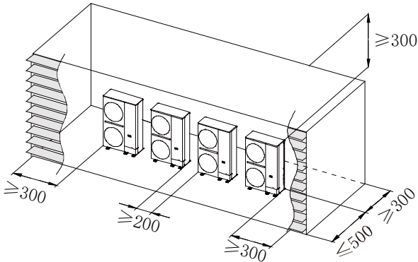
Figure 2-3.20: More than one outdoor unit installation (unit: mm)
