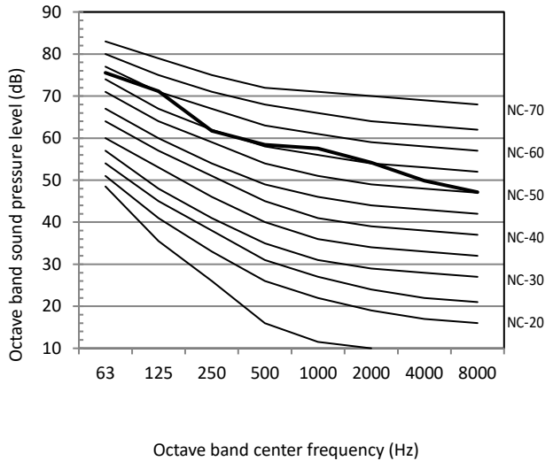
Figure 2-10.4: 18HP octave band level
