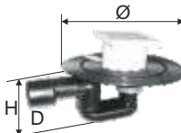
Sifon PP teras gr tar cu ie ire PP terrace trap with grid, "reduced encumbrance" version outlet
