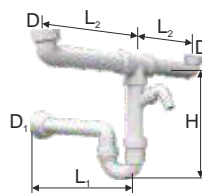
Sifon alb PP pentru sp lator dublu cu racord la ma ina de sp lator Double sink trap with washing machine connection - white PP
