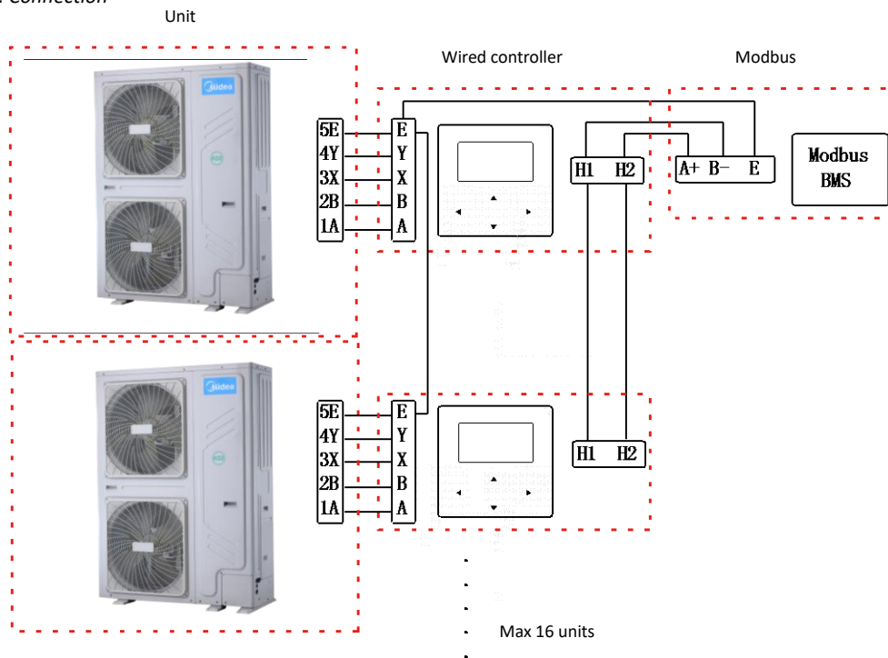
Figure 4-2.7: Wiring
