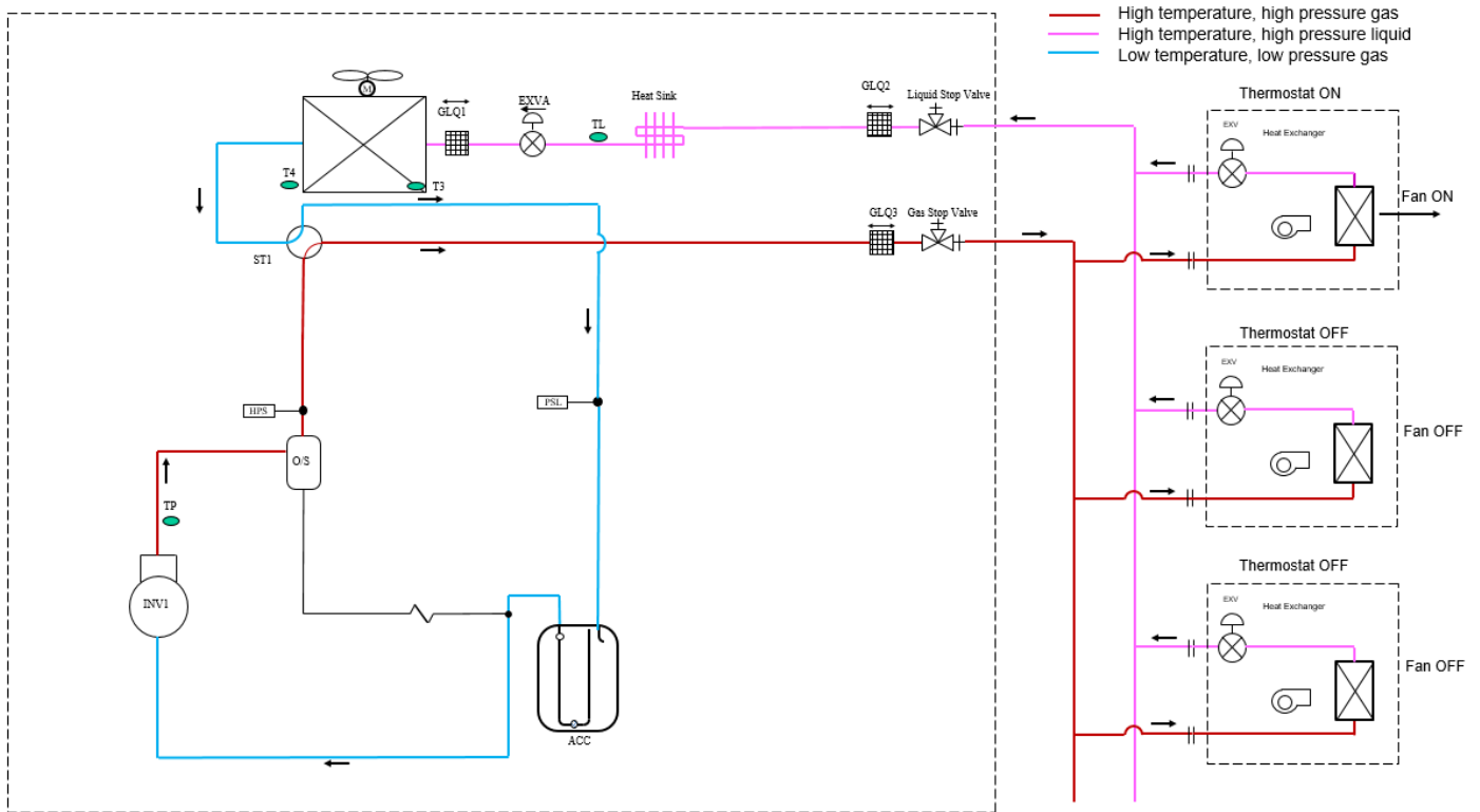
Figure 2-3.7: Refrigerant flow during heating operation
