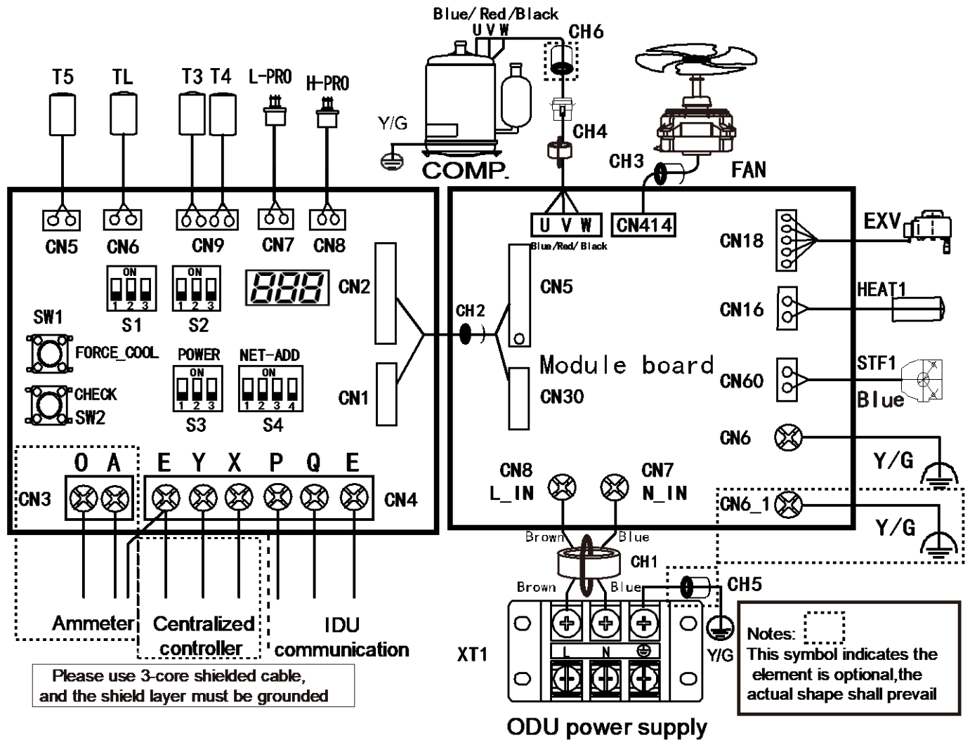
Figure 4-3.1: 8kW Outdoor units wiring diagram
