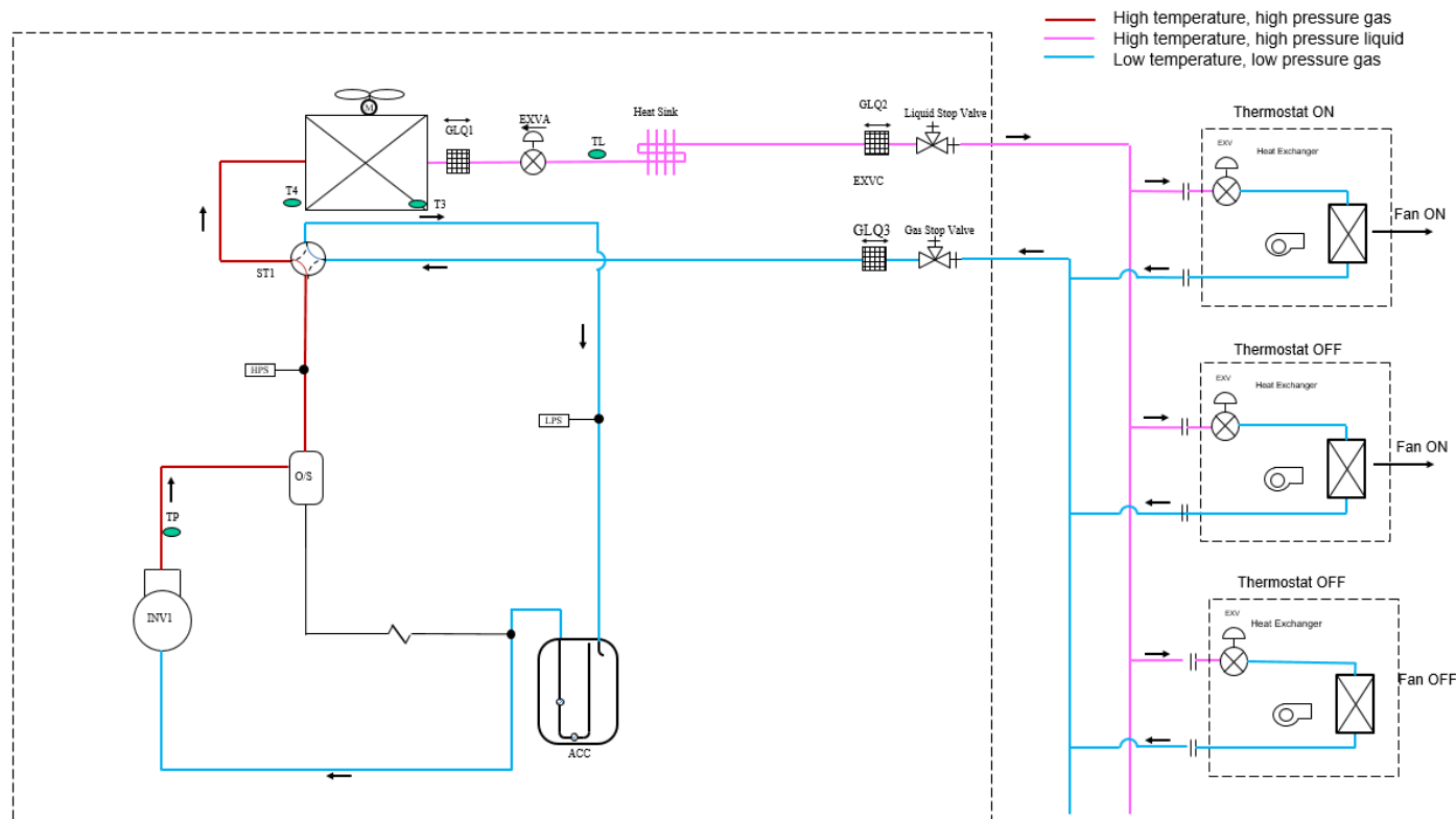
Figure 2-3.1: Refrigerant flow during cooling operation
