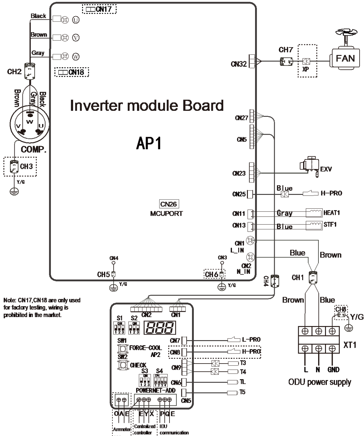
Figure 4-3.1: 10-16kW Outdoor units wiring diagram
