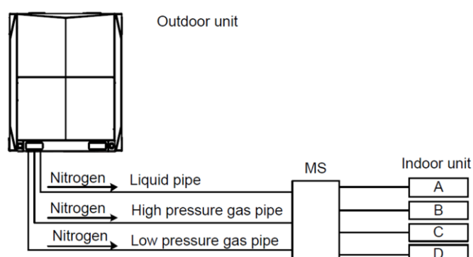
Figure 3-5.13: Gastightness test
