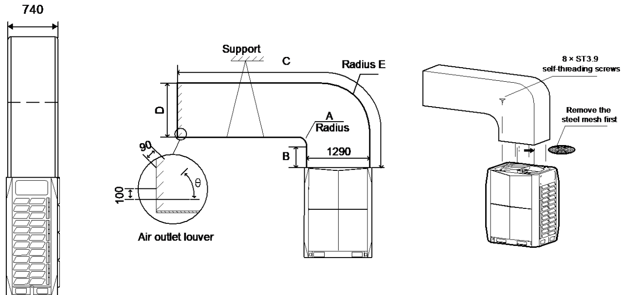
Figure 3-3.5: Longitudinal ducting for 14/16/18HP units (unit: mm)
