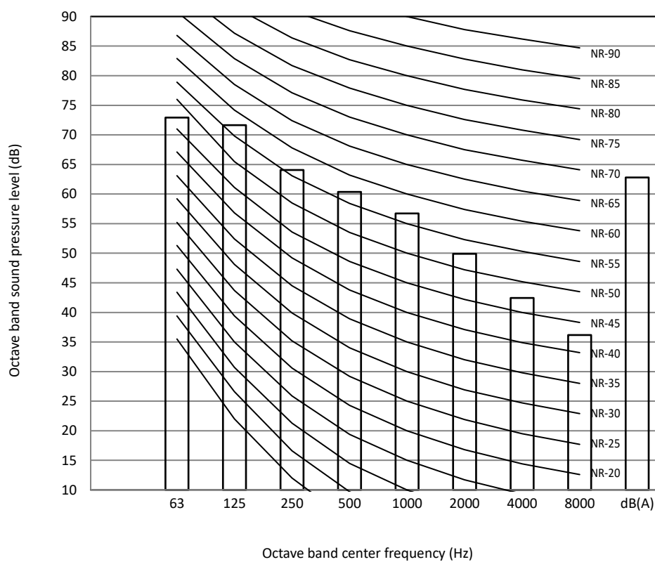
Figure 2-11.5: 14HP octave band level
