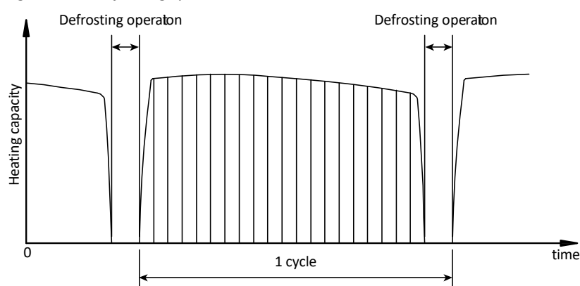
Figure 2-9.3: Defrosting cycle
