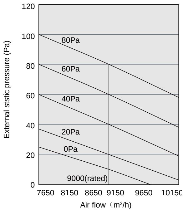
Figure 3-3.6: 8HP units fan performance
