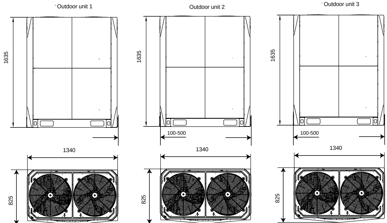
Figure 2-2.8: 46/48/50/52/54HP dimensions (unit: mm)
