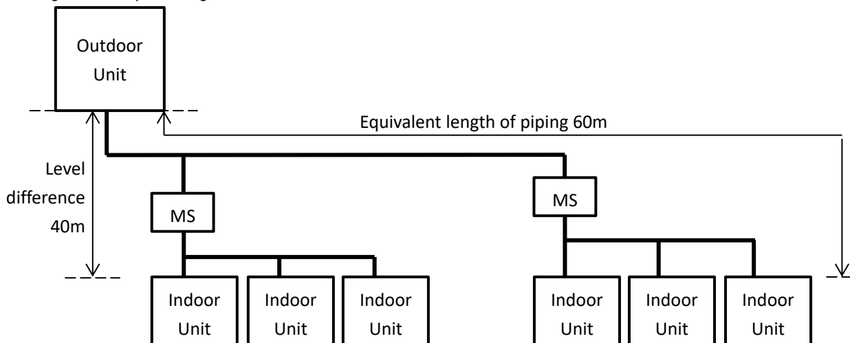
Figure 1-6.2: System diagram
