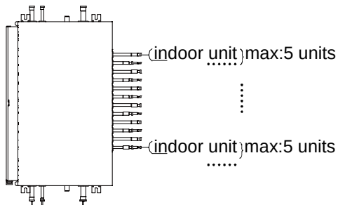
Figure 3-4.8: MS Connecting to indoor unit ≤ 16kW
