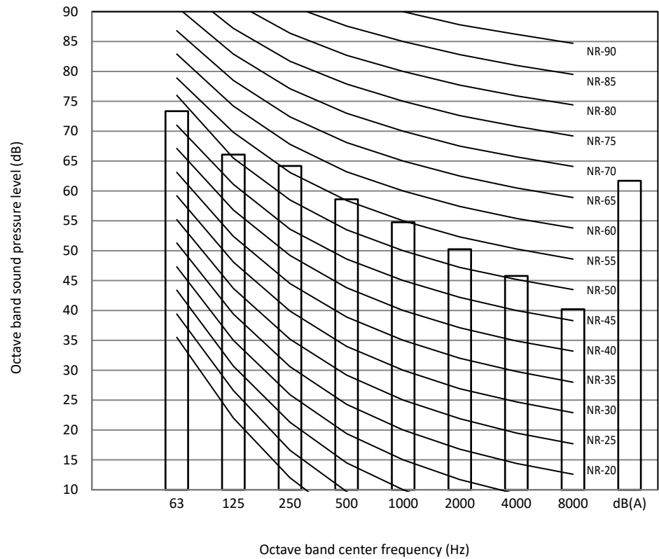
Figure 2-11.5: 14HP octave band level
