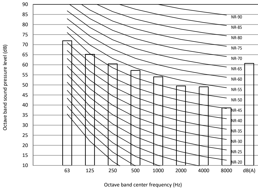
Figure 2-11.3: 10HP octave band level
