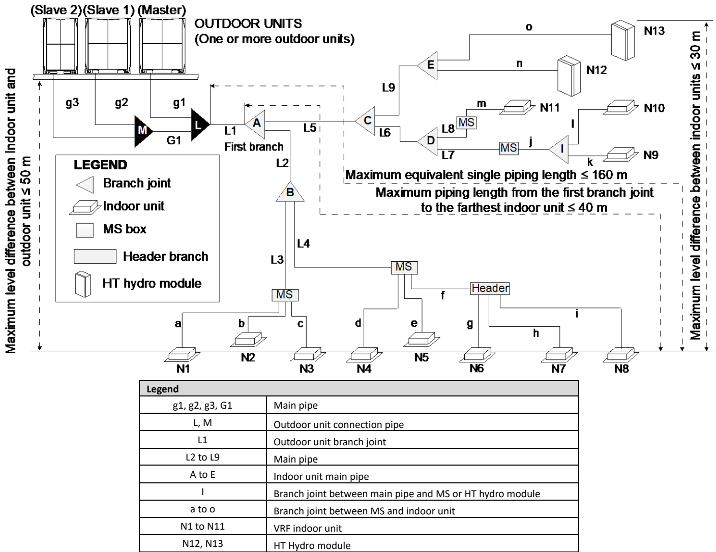
Figure 3-4.3: Permitted refrigerant piping lengths and level differences
