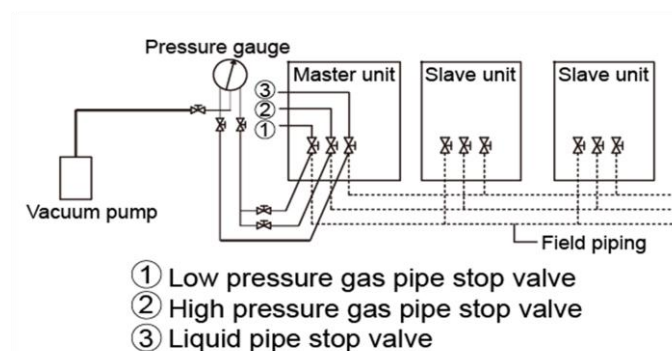
Figure 3-5.14: Vacuum drying
