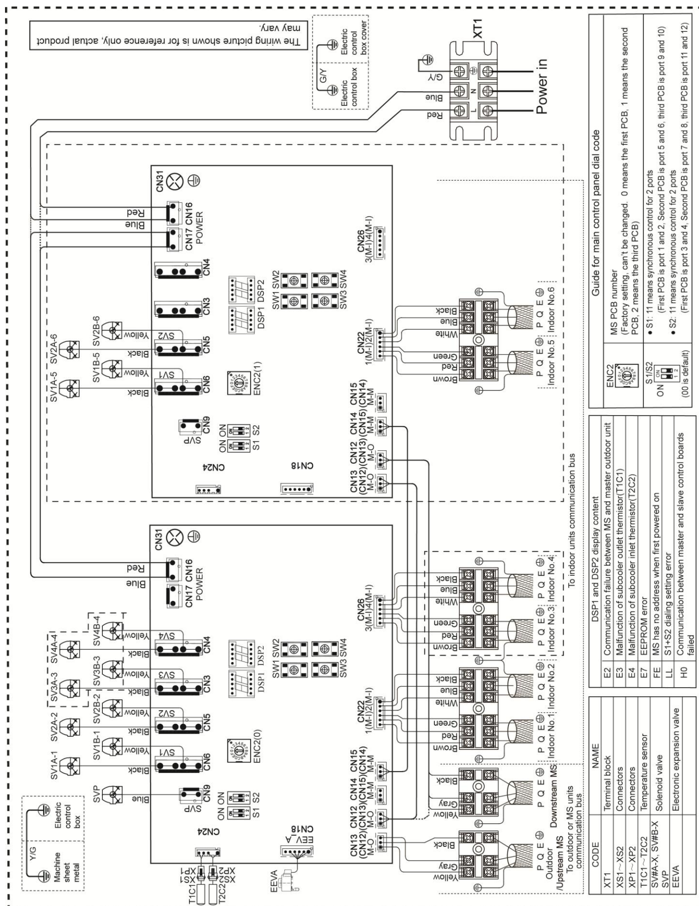
Figure 2-6.3: MS04/MS06 wiring diagram
