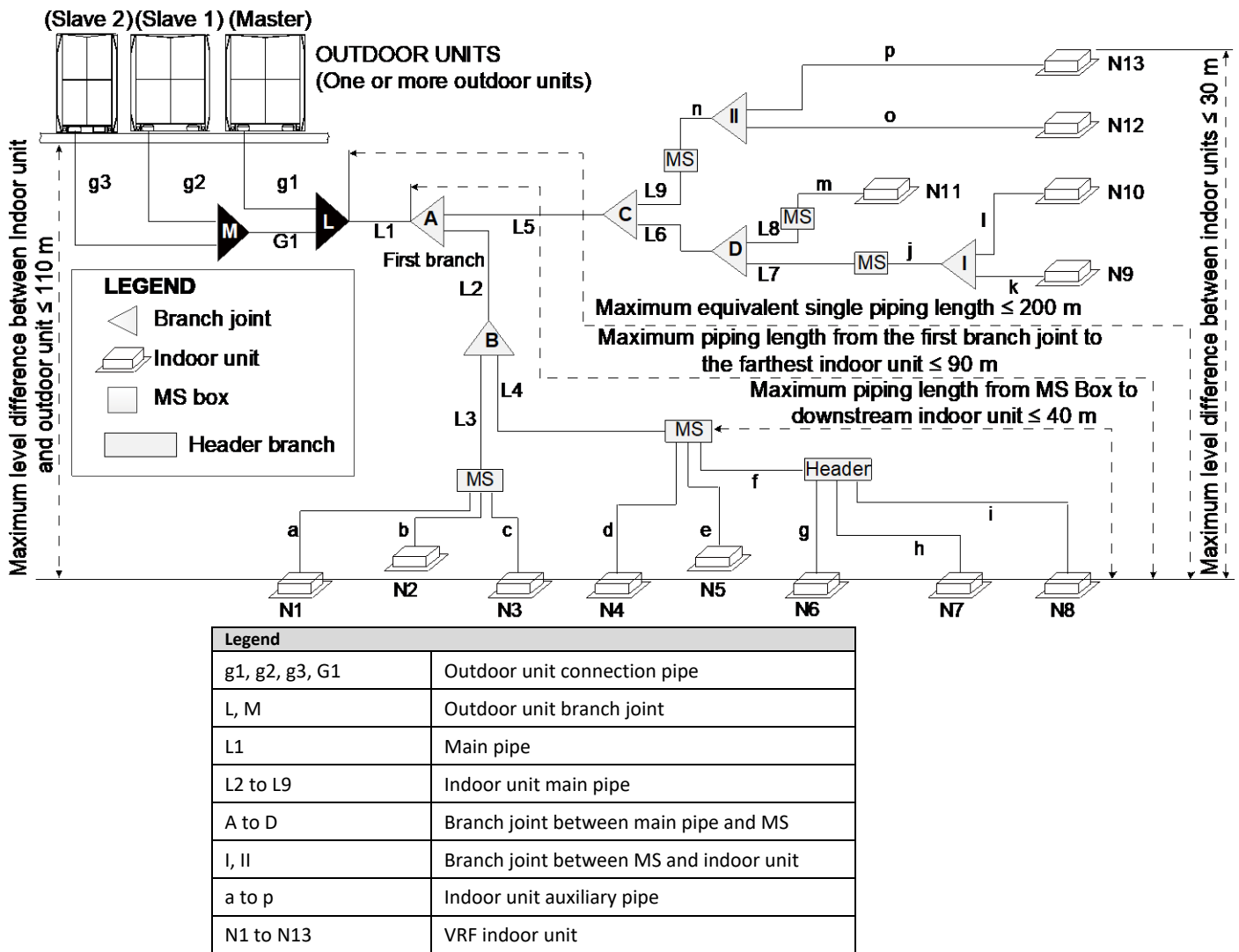
Figure 3-4.2: Permitted refrigerant piping lengths and level differences
