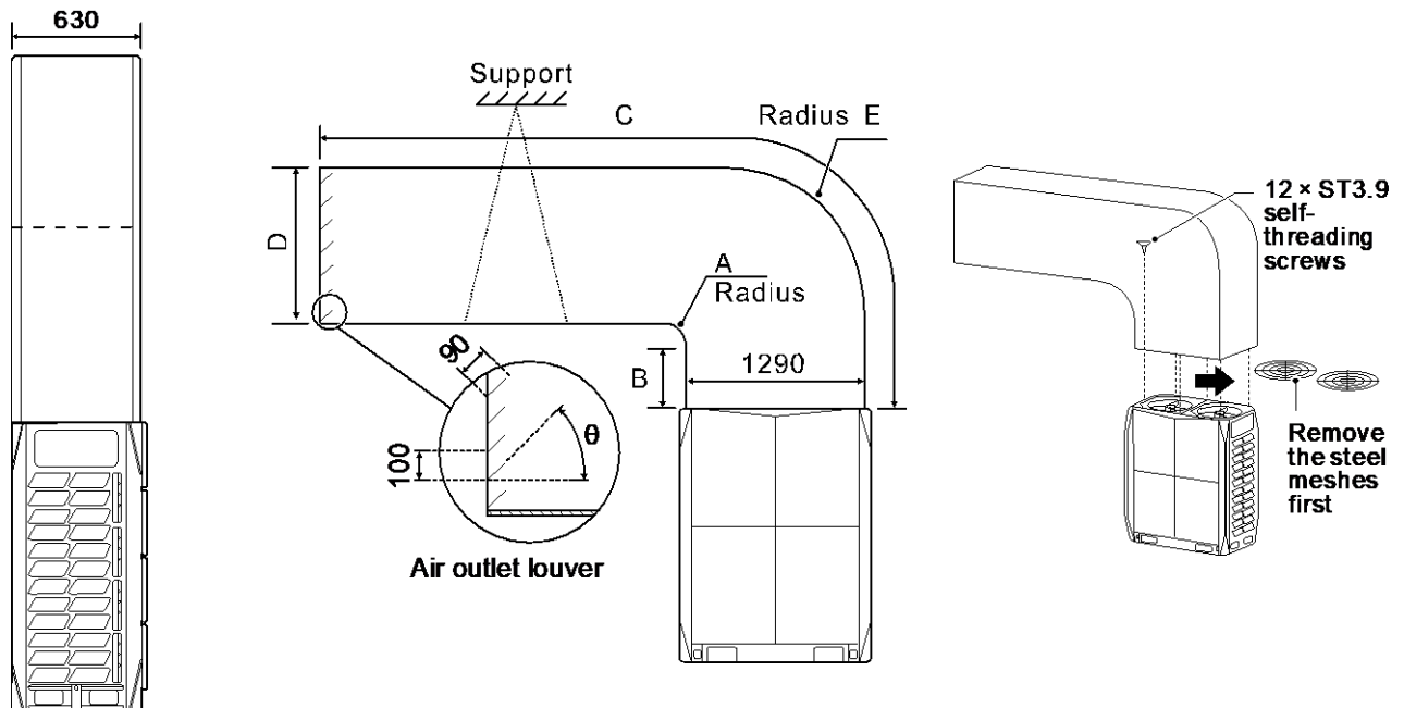
Figure 3-3.5: Longitudinal ducting for 14/16/18HP units (unit: mm)
