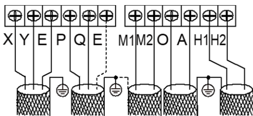
Figure 3-9.11: Outdoor unit communication terminals
