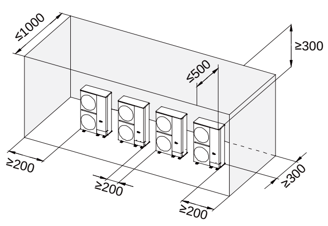
Figure 2-3.4: More than one outdoor unit installation (unit: mm)
