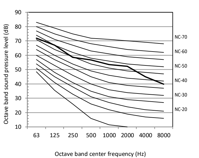
Figure 2-10.5: 14HP octave band level
