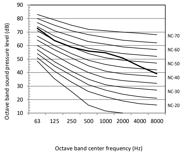
Figure 2-10.3: 10HP octave band level
