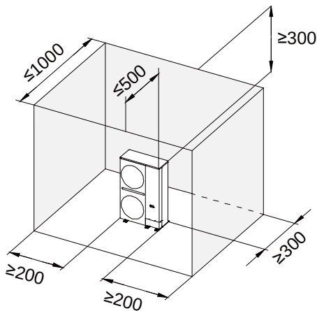
Figure 2-3.3: One outdoor unit installation (unit: mm)
