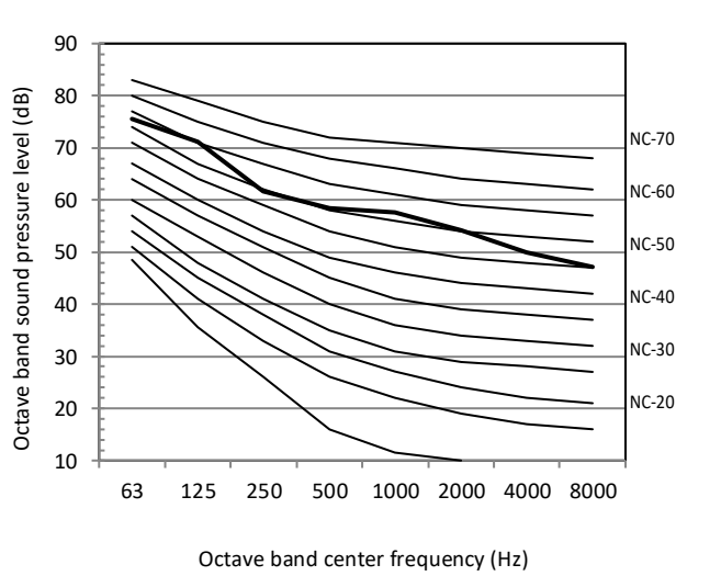
Figure 2-10.7: 18HP octave band level
