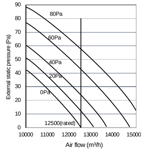
Figure 3-3.5: 14HP units fan performance
