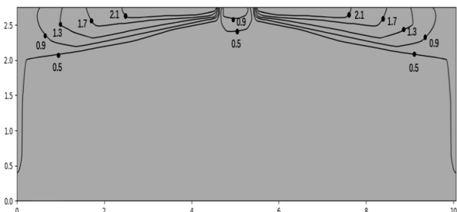
Figure 9.15: MIH100Q4N18 cooling at 300s
