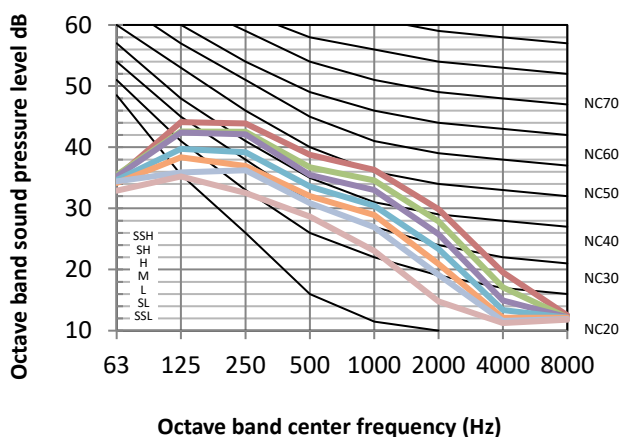
Figure 8.10: MIH112Q4N18 octave band levels
