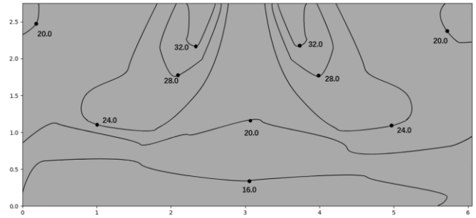
Figure 9.28: MIH56Q4N18 heating at 300s
