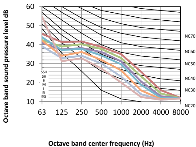
Figure 8.8: MIH90Q4N18 octave band levels
