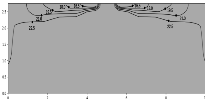
Figure 9.33: MIH90Q4N18 cooling at 300s
