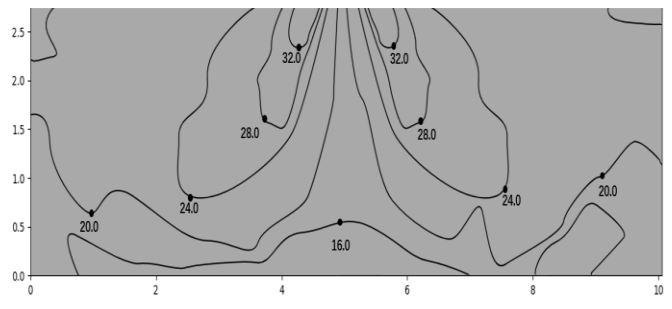
Figure 9.40: MIH140Q4N18 heating at 300s
