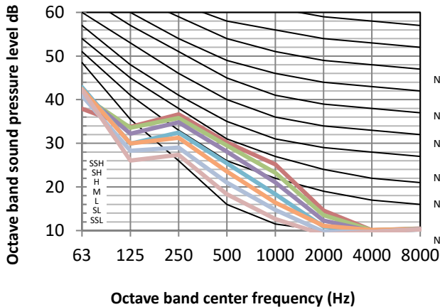
Figure 8.4: MIH45Q4N18 octave band levels
