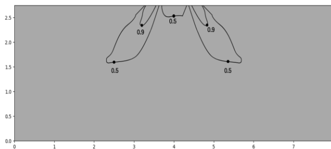
Figure 9.10: MIH71Q4N18 heating at 300s
