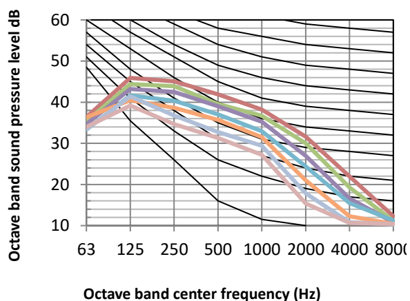
Figure 8.11: MIH140Q4N18 octave band levels
