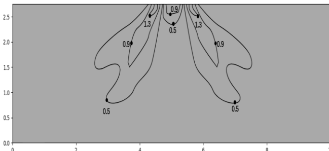
Figure 9.16: MIH100Q4N18 heating at 300s
