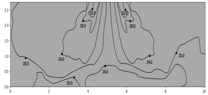
Figure 9.38: MIH112Q4N18 heating at 300s
