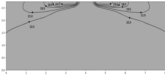
Figure 9.29: MIH71Q4N18 cooling at 300s
