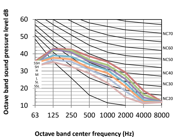
Figure 8.9: MIH100Q4N18 octave band levels
