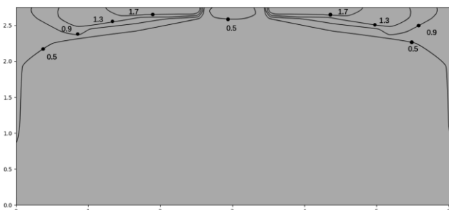
Figure 9.5: MIH45Q4N18 cooling at 300s
