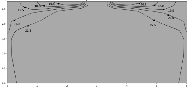
Figure 9.27: MIH56Q4N18 cooling at 300s
