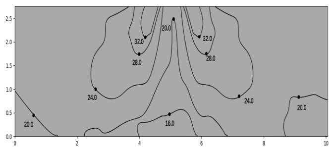
Figure 9.40: MIH140Q4N18 heating at 300s
