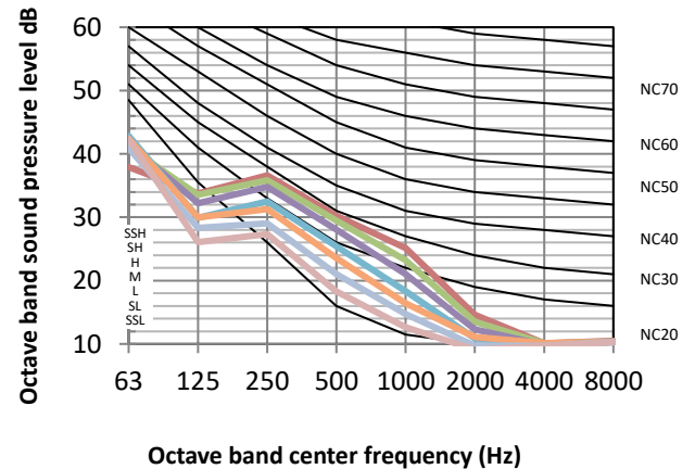
Figure 8.5: MIH56Q4N18 octave band levels
