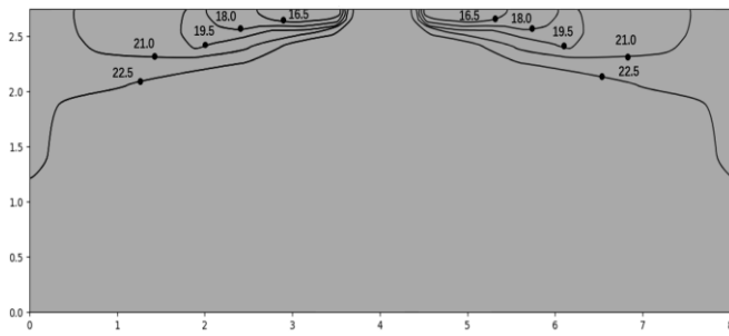
Figure 9.31: MIH80Q4N18 cooling at 300s
