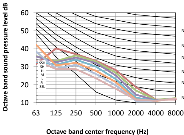
Figure 8.4: MIH45Q4N18 octave band levels
