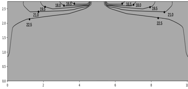
Figure 9.37: MIH112Q4N18 cooling at 300s
