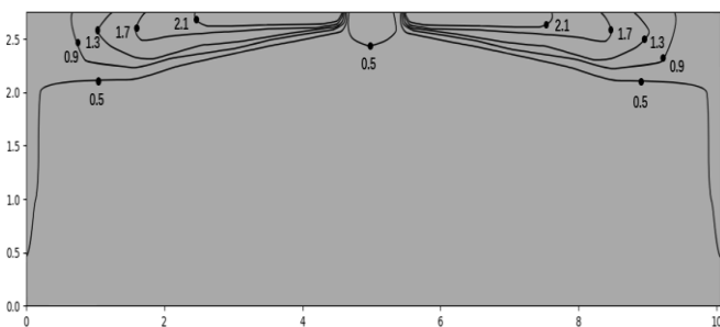
Figure 9.15: MIH100Q4N18 cooling at 300s
