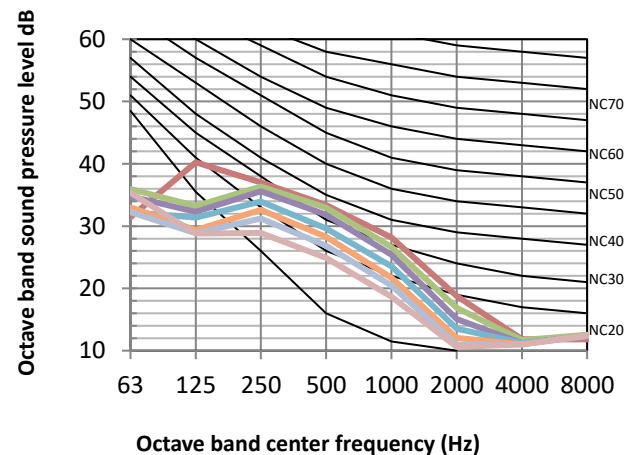
Figure 8.5: MIH56Q4N18 octave band levels
