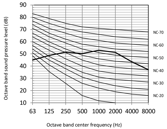
Figure 2-10.3: 100 model octave band level
