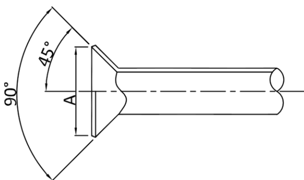
Figure 3-4.2: Flared opening
