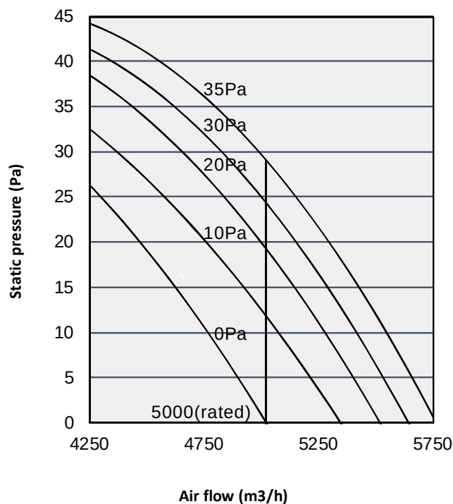
Figure 3-2.7: 120/140/160 model units fan performance
