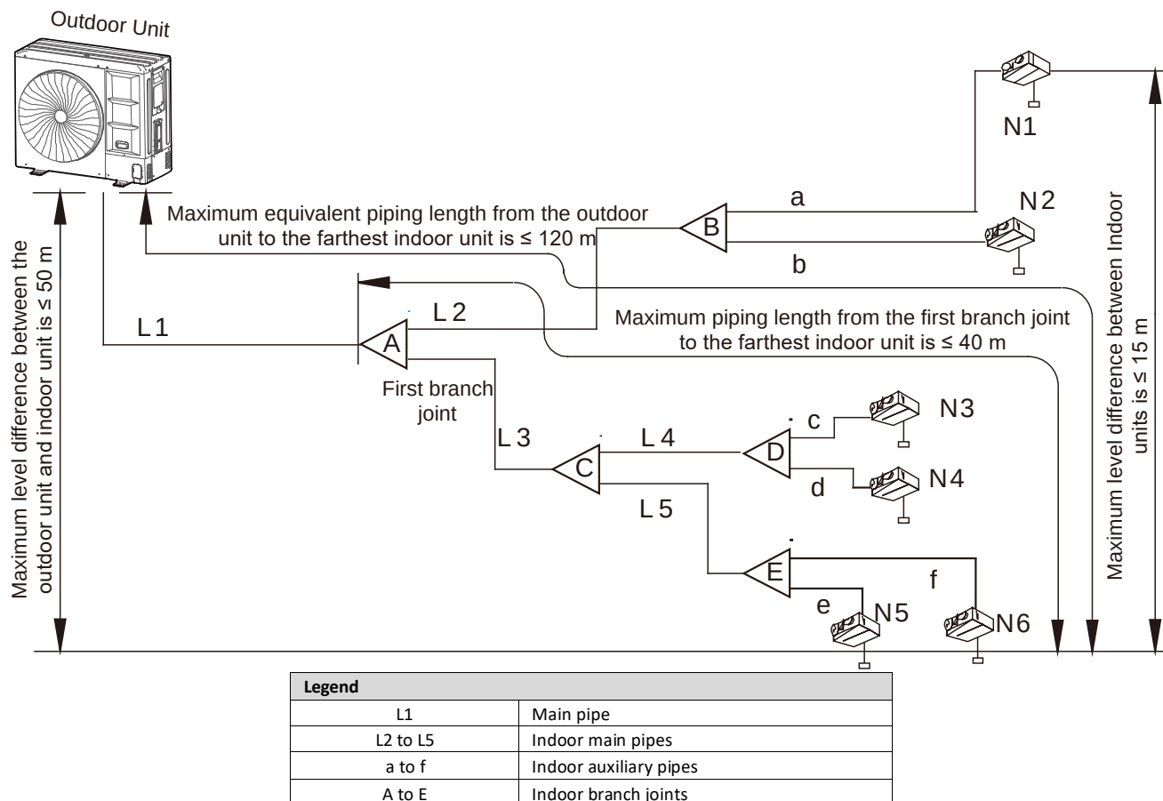
Figure 3-3.1: Permitted refrigerant piping lengths and level differences
