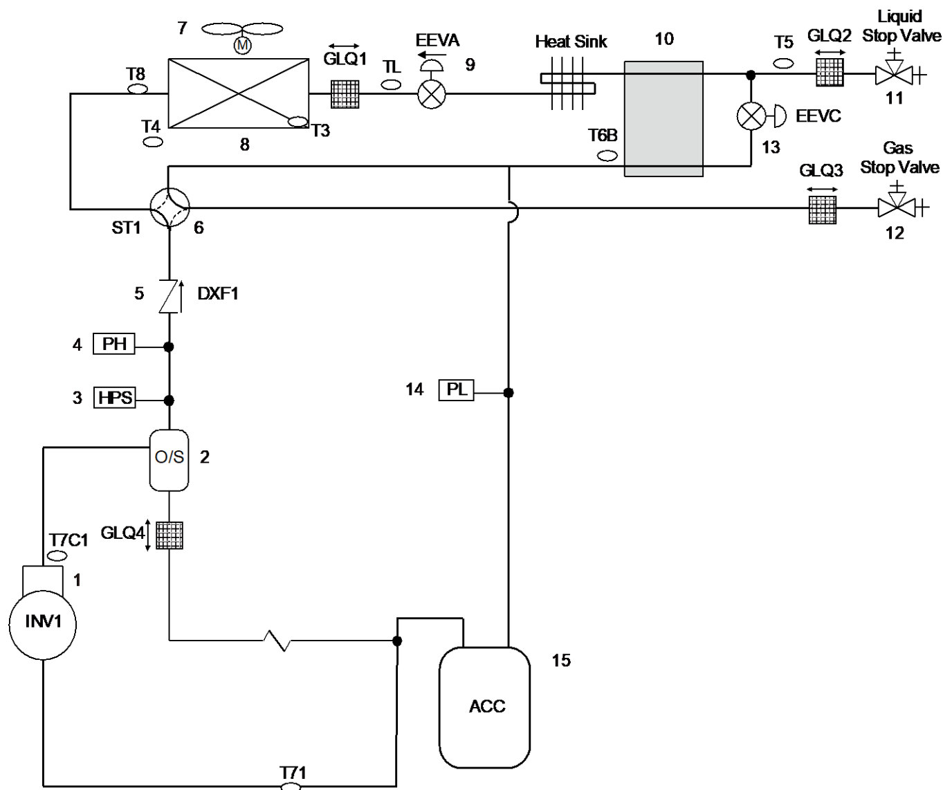
Figure 2-4.1: 80/100 model piping diagram
