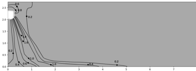
Figure 9.14: MIH71GN18 heating at 300S
