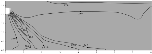
Figure 9.27: MIH56GN18 cooling at 300S
