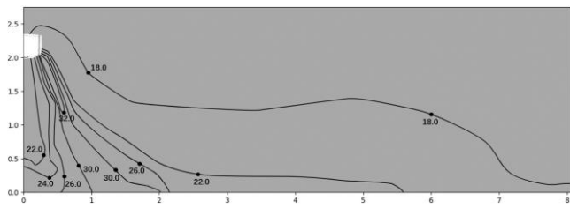
Figure 9.30: MIH71GN18 heating at 300S
