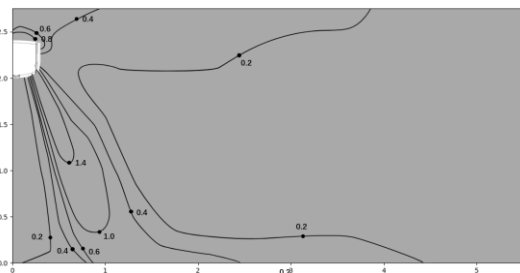
Figure 9.10: MIH45GN18 heating at 300S
