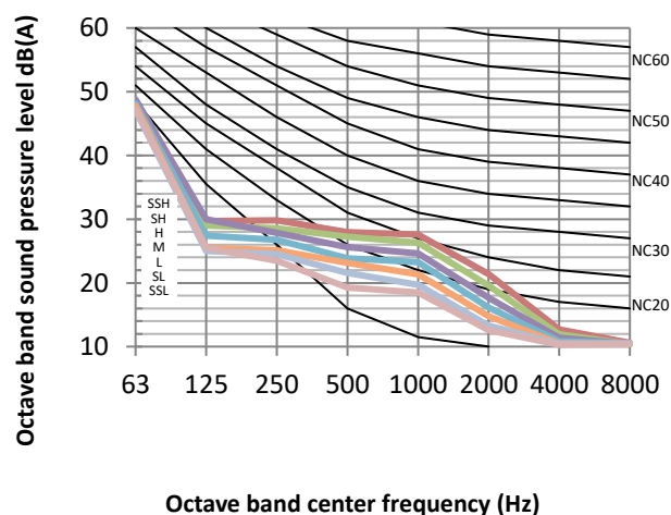
Figure 8.3: MIH22GN18 octave band levels
