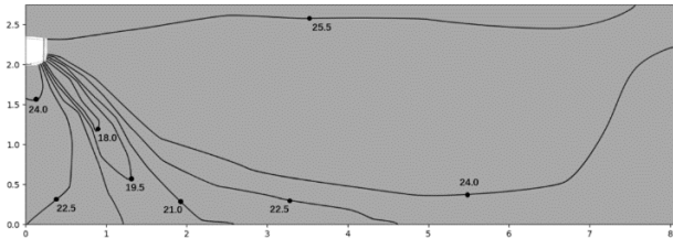
Figure 9.31: MIH80GN18 cooling at 300S
