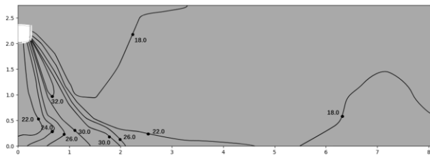
Figure 9.28: MIH56GN18 heating at 300S
