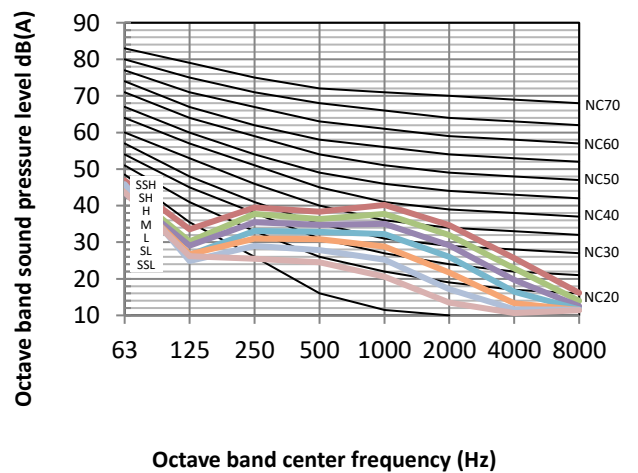
Figure 8.9: MIH80GN18 octave band levels
