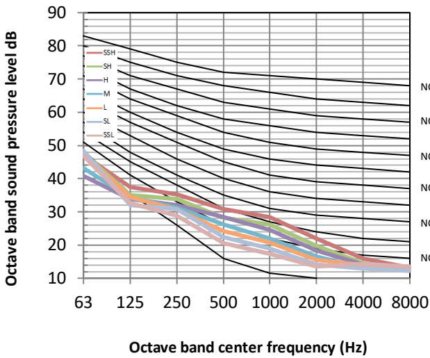
Figure 8.5: MIH28T3N18 octave band levels
