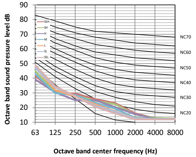
Figure 8.4: MIH22T3N18 octave band levels
