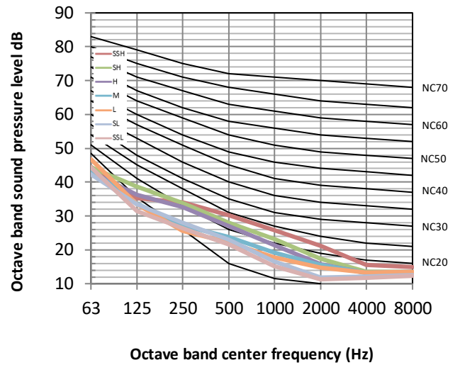
Figure 8.6: MIH36T3N18 octave band levels
