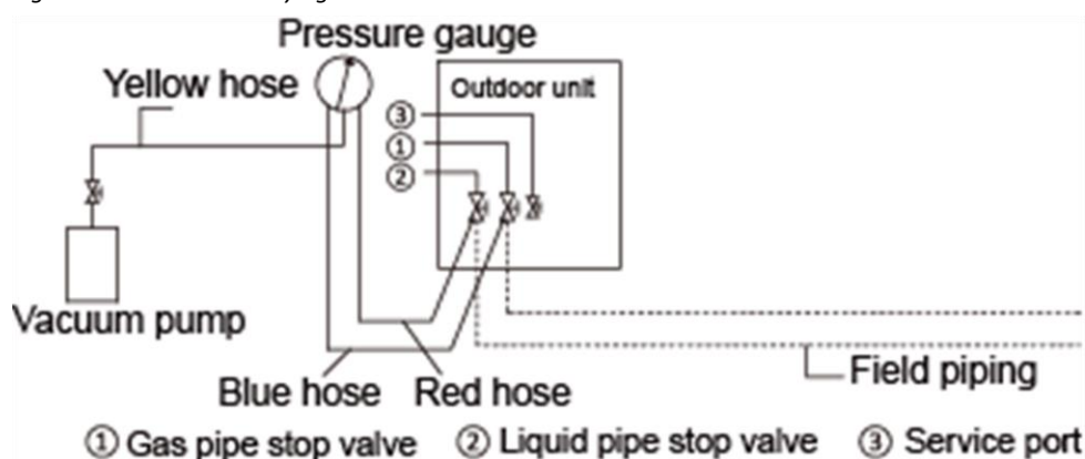
Figure 3-5.15: Vacuum drying
