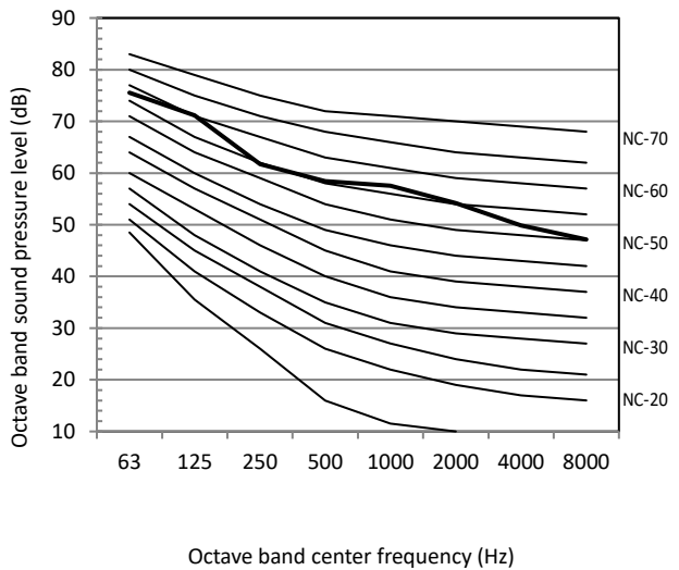
Figure 2-10.4: 18HP octave band level
