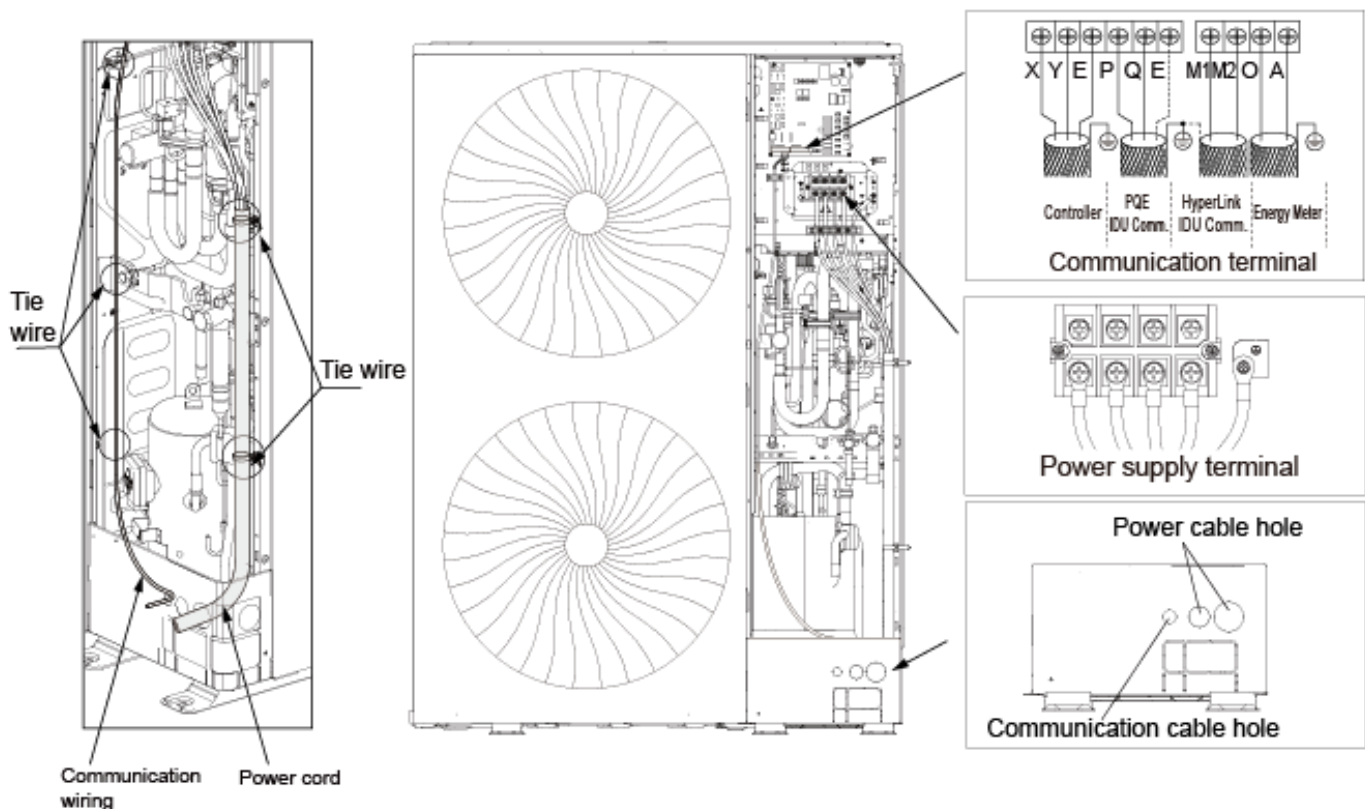
Figure 3-9.1: Wiring layout
