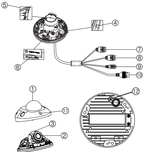
Figure 8: IP fixed lens wedge camera
