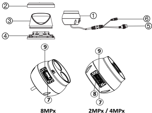
Figure 3: IP fixed lens turret camera
