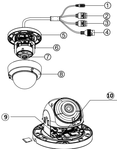
Figure 5: IP fixed lens dome camera
