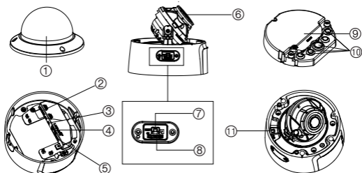
Figure 6: IP motorized lens dome camera
