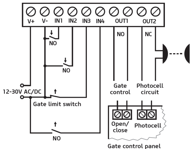
Wiring for one gate with photocell and position limit switch (control mode 3)
