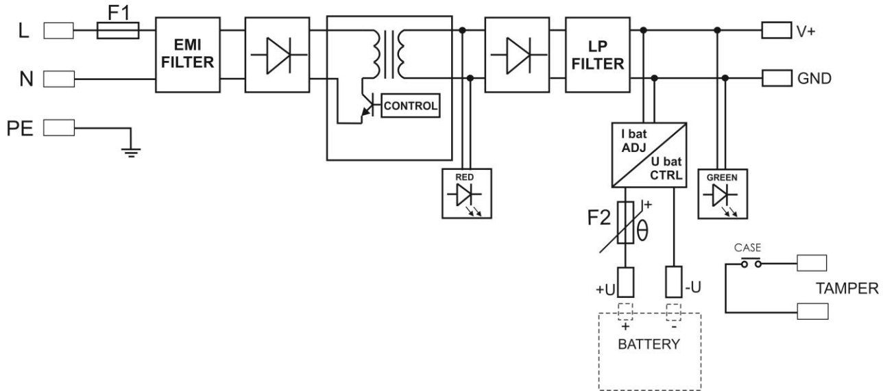
Fig.1. The block diagram of the PSU.
